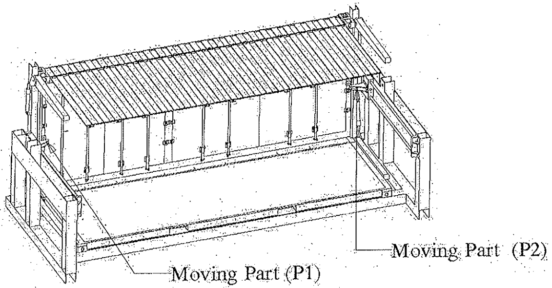
Figure 3: Transport container after the first folding step
