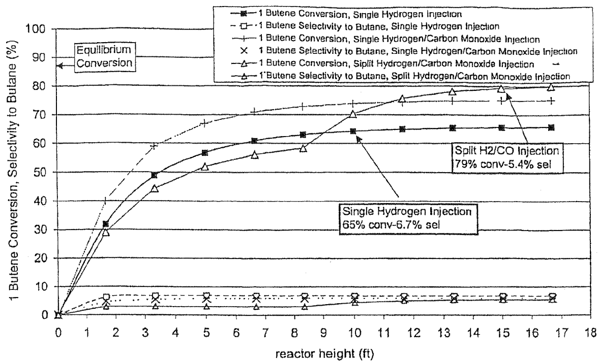
Figure 14: Effect of CO and partial injections on 1-Butene conversion and selectivity
