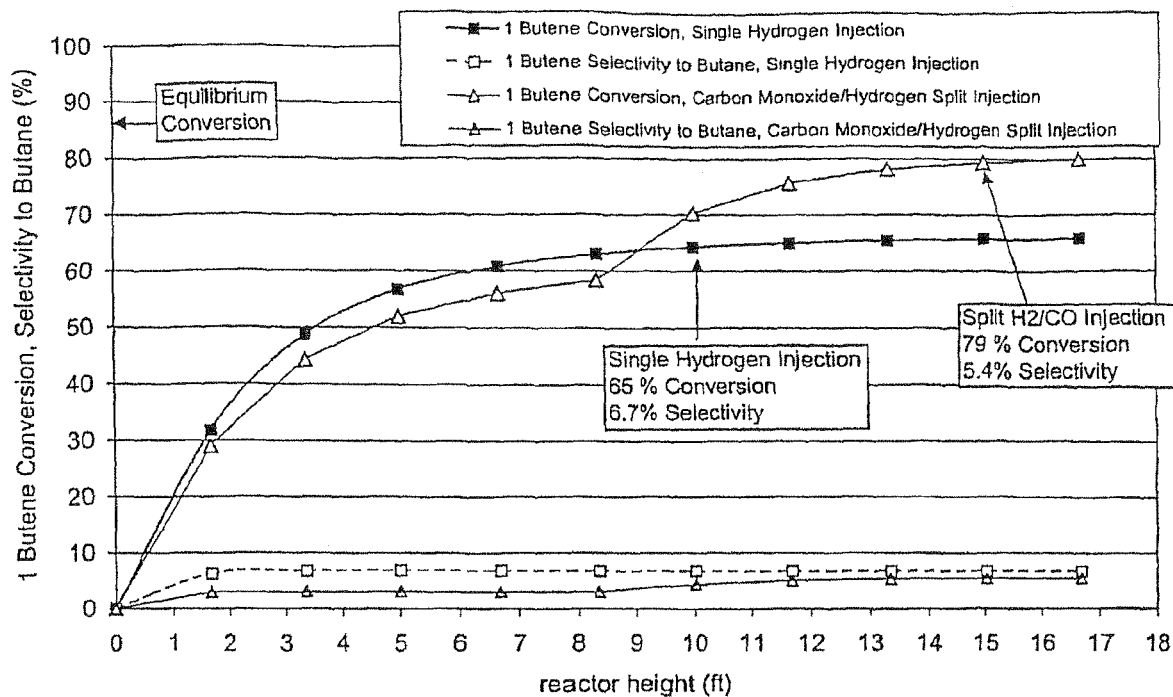
Figure 12: Effect of H 2 injections on 1-Butene conversion and selectivity
