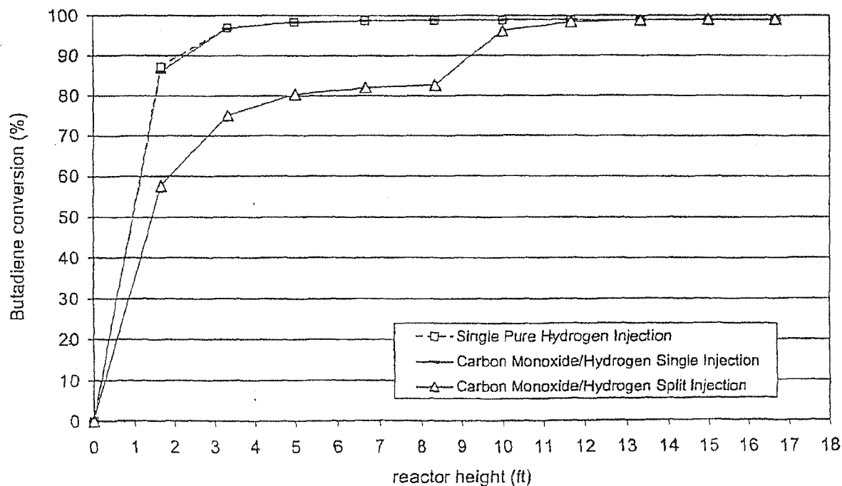
Figure 13: Effect of CO and partial injections on BD conversion
