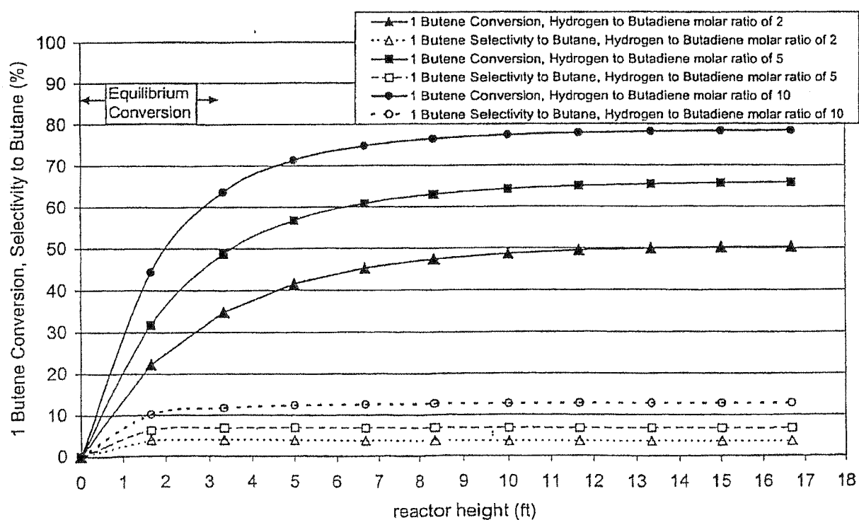
Figure 11: Effect of H 2 flow rate on 1-Butene conversion and selectivity
