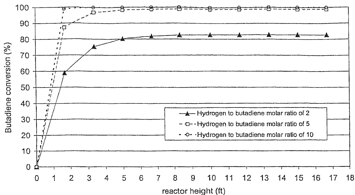
Figure 10: Effect of H 2 flow rate on butadiene conversion
