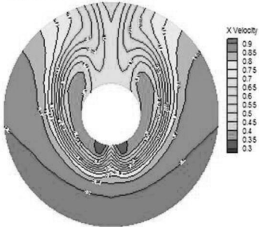
Wake contour w/o VG
