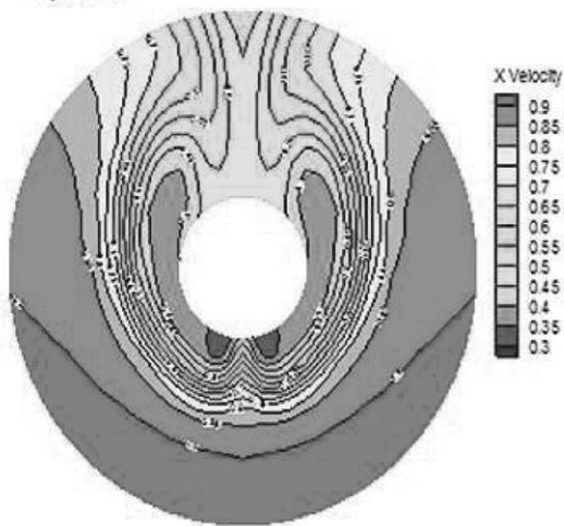
Wake contour w/o VG
