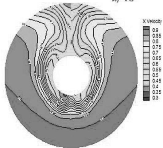
Wake contour w/ VG
