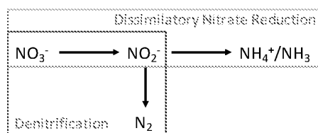
Scheme 1: Denitrification and DNRA pathways
