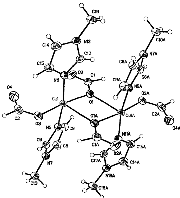
Molecular Structure of [\text{Cu}(\text{1-methylimidazole})_2(\text{HCOO})_2]_2
