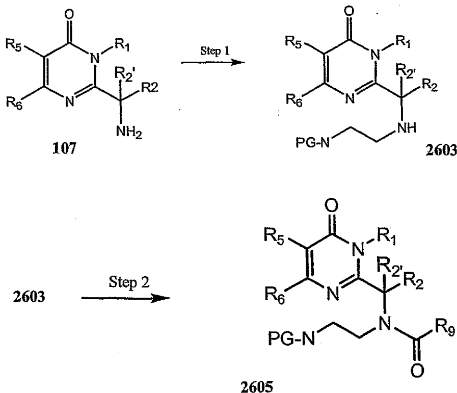
Reaction Scheme 26
