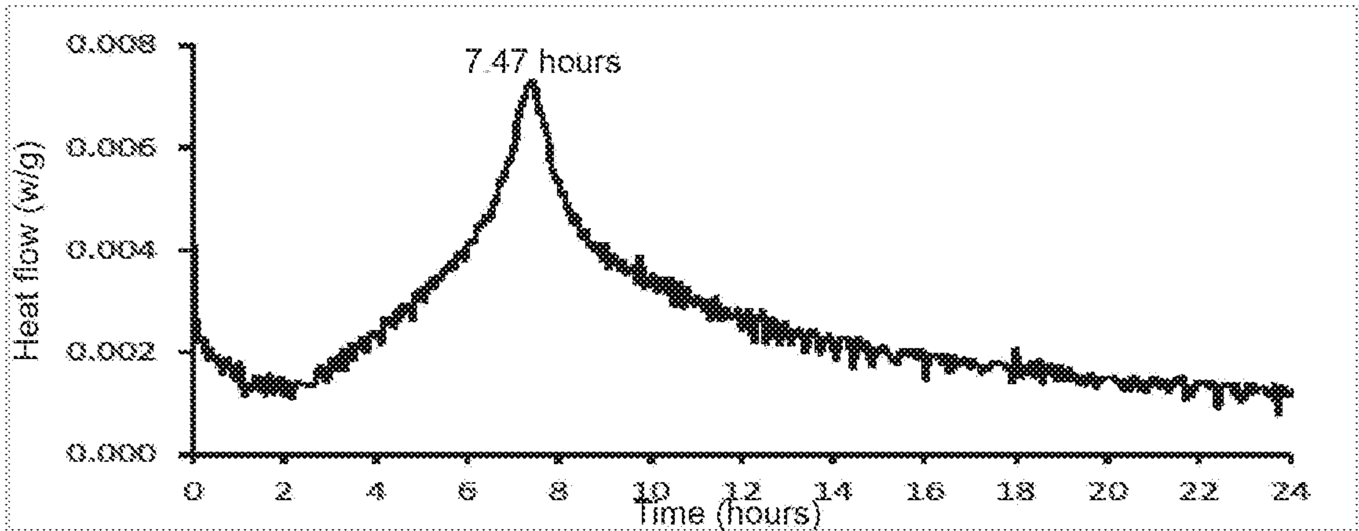
Figure 1B:Heat flow curve of the CEMI 52.5R cement mixture - sample Ex.3 L2
