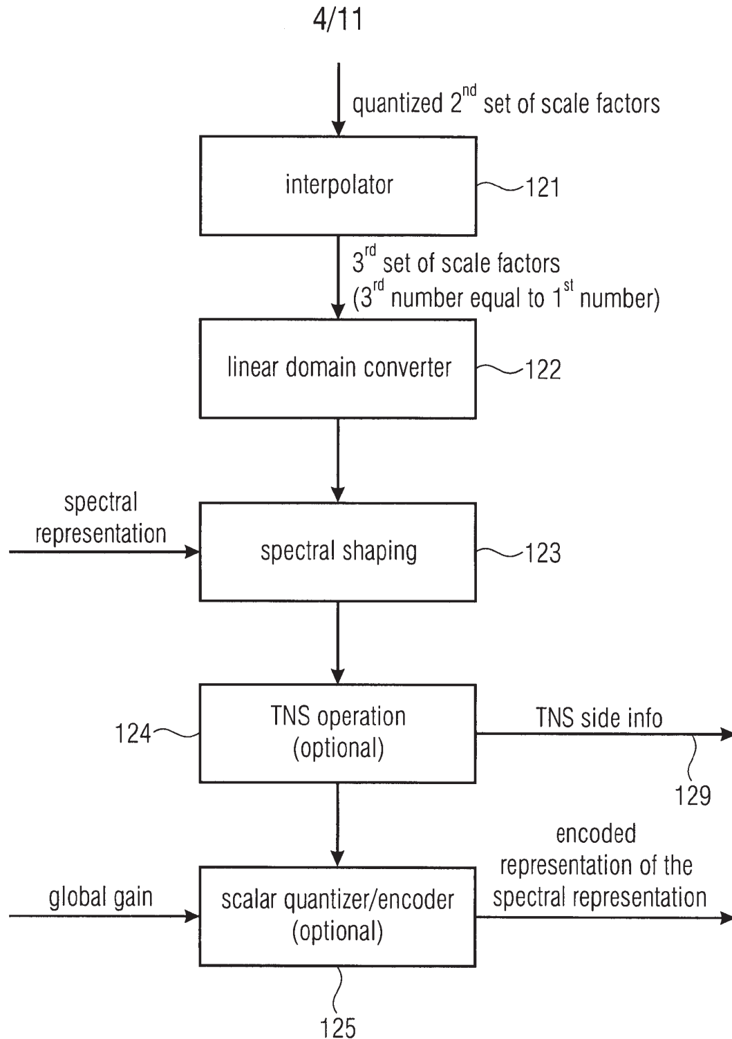
Fig. 5 (SPECTRAL PROCESSOR)
