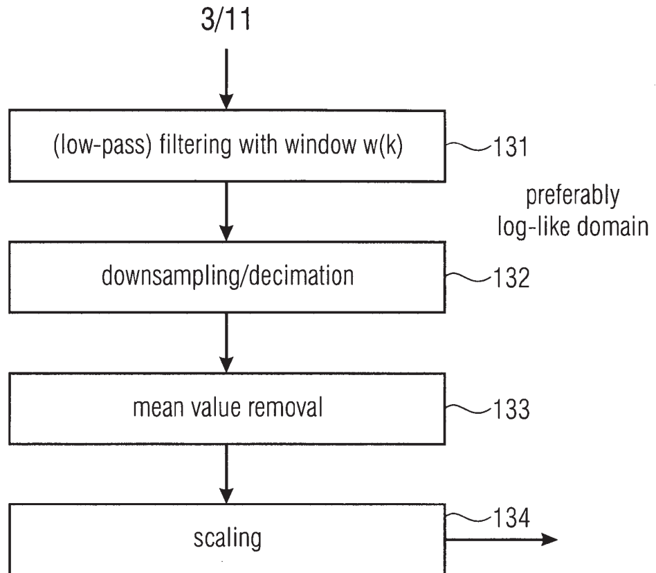
Fig. 3 (DOWNSAMPLER)
