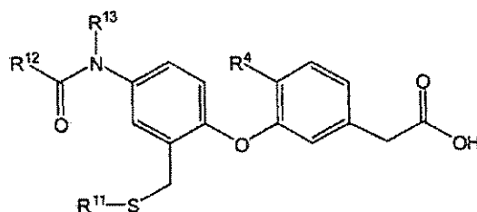
Formula (III).
