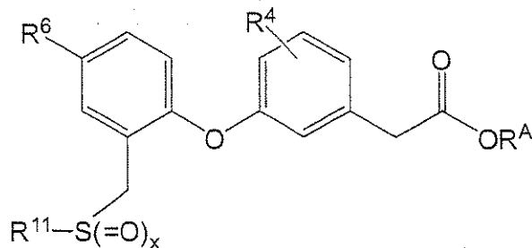
Formula (I)
