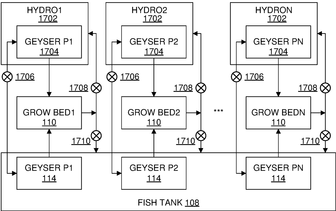
FIG. 17 AQUAPONICS/HYDRO ON DEMAND 1700
