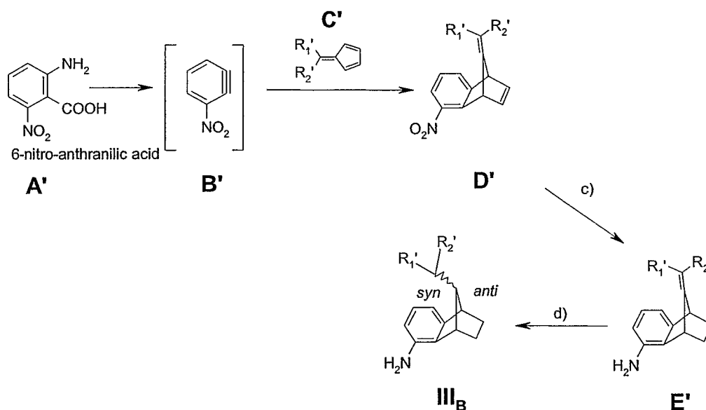
Scheme 1: Synthesis of III B using 6-nitroanthranilic acid
