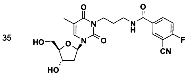
30 3-Cyano-N-((2R,3R)-2,3-dihydroxy-4-[3-((2R,4S,5R)-4-hydroxy-5-hydroxymethyl-tetrahydro-furan-2-yl)-5-methyl-2,6-dioxo-3,6-dihydro-2H-pyrimidin-1-yl]-butyl)-4-fluoro-benzamide
