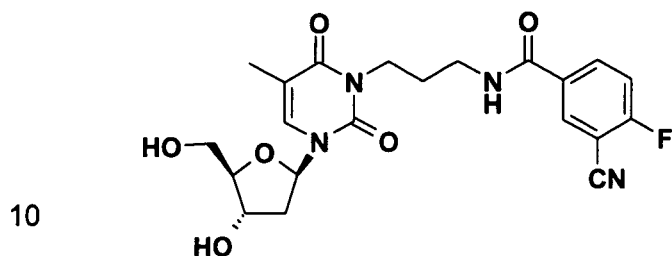
3-Cyano-4-[F]fluoro-N-(thymidiny-propyl)-benzamide
