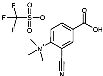
Trifluoro-methanesulfonate(4-carboxy-2-cyano-phenyl)-trimethyl-ammonium;
