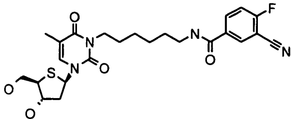
3-Cyano-4-fluoro-N-{6-[3-((2R,4S,5R)-4-hydroxy-5-hydroxymethyl-tetrahydro-thiophen-2-yl)-5-methyl-2,6-dioxo-3,6-dihydro-2H-pyrimidin-1-yl]-hexyl}-benzamide
