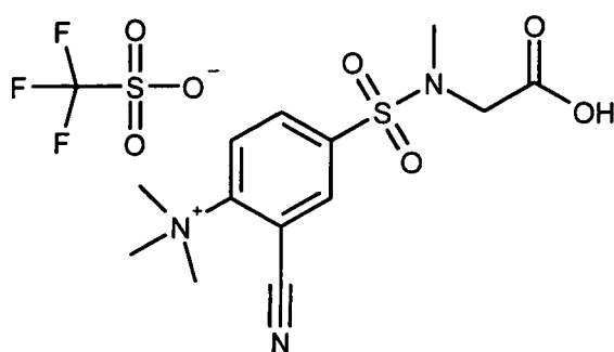
Trifluoro-methanesulfonate[4-(carboxymethyl-methyl-sulfamoyl)-2-cyano-phenyl]-trimethyl-ammonium;
