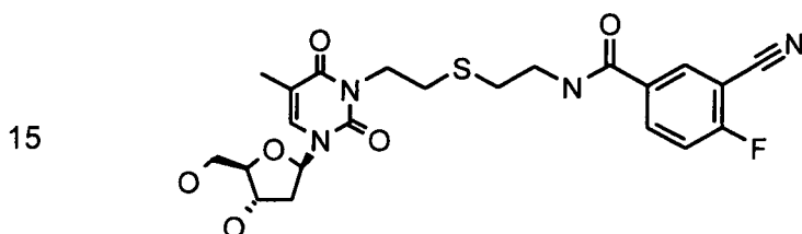
20 3-Cyano-4-fluoro-N-(2-{2-[3-((2R,4S,5R)-4-hydroxy-5-hydroxymethyl-tetrahydro-furan-2-yl)-5-methyl-2,6-dioxo-3,6-dihydro-2H-pyrimidin-1-yl]-ethylsulfanyl}-ethyl)-benzamide
