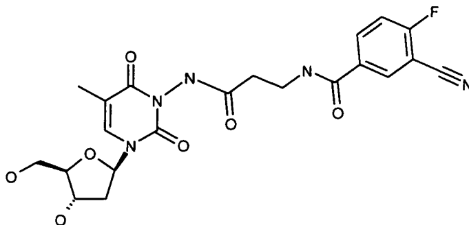
3-Cyano-4-fluoro-N-{2-[3-((2R,4S,5R)-4-hydroxy-5-hydroxymethyl-tetrahydro-furan-2-yl)-5-methyl-2,6-dioxo-3,6-dihydro-2H-pyrimidin-1-yl]-ethyl}-benzamide
