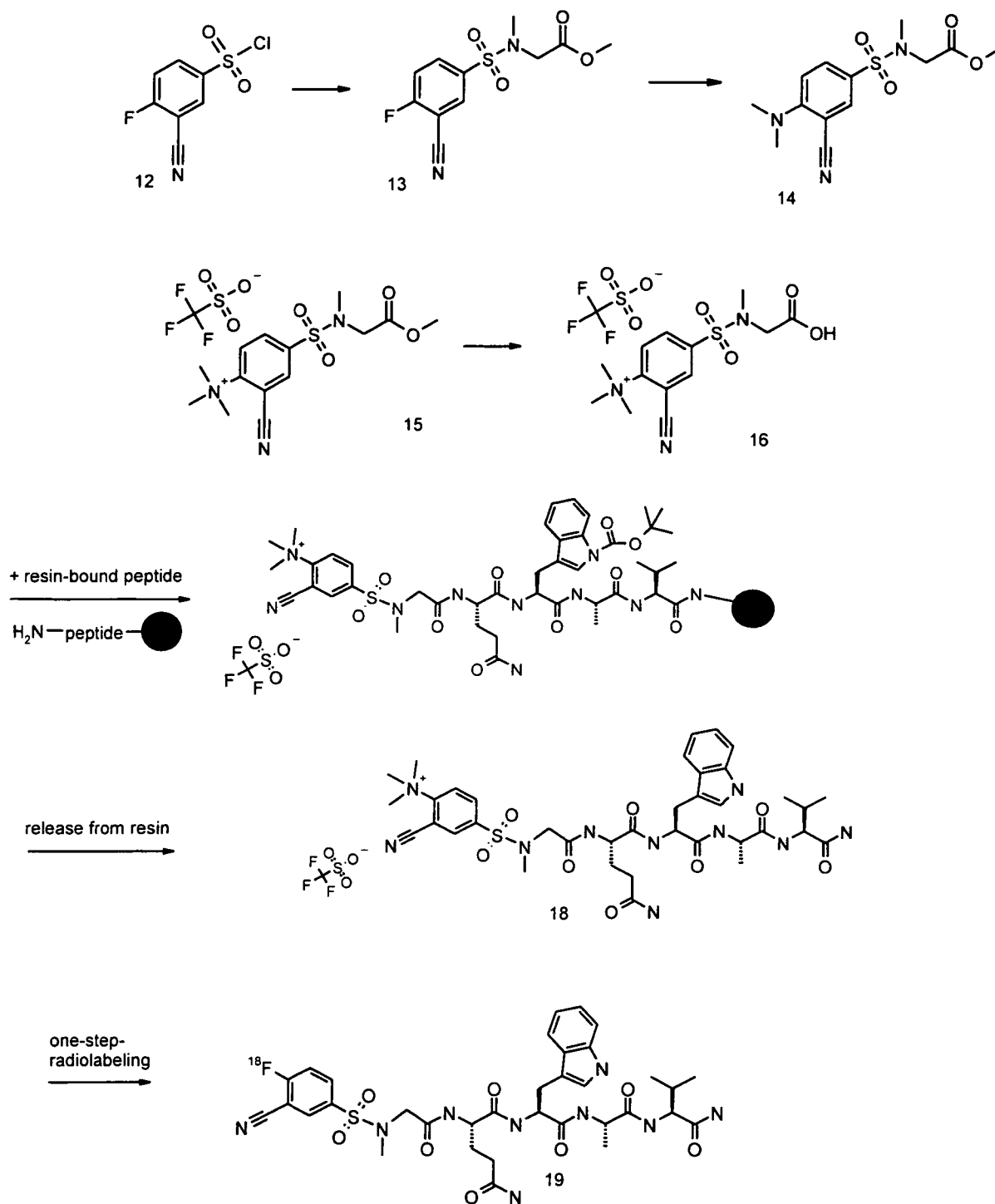
Scheme 4
