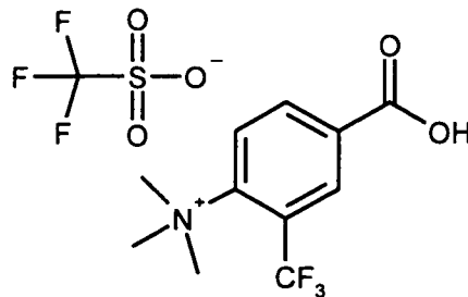
Trifluoro-methanesulfonate(4-carboxy-2-trifluoromethyl-phenyl)-trimethyl-ammonium;
