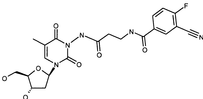
3-Cyano-4-fluoro-N-{2-[3-((2R,4S,5R)-4-hydroxy-5-hydroxymethyl-tetrahydro-furan-2-yl)-5-methyl-2,6-dioxo-3,6-dihydro-2H-pyrimidin-1-ylcarbonyl]-ethyl}-benzamide
