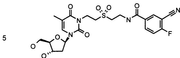
10 3-Cyano-4-fluoro-N-(2-{2-[3-((2R,4S,5R)-4-hydroxy-5-hydroxymethyl-tetrahydro-furan-2-yl)-5-methyl-2,6-dioxo-3,6-dihydro-2H-pyrimidin-1-yl]-ethanesulfonyl}-ethyl)-benzamide
