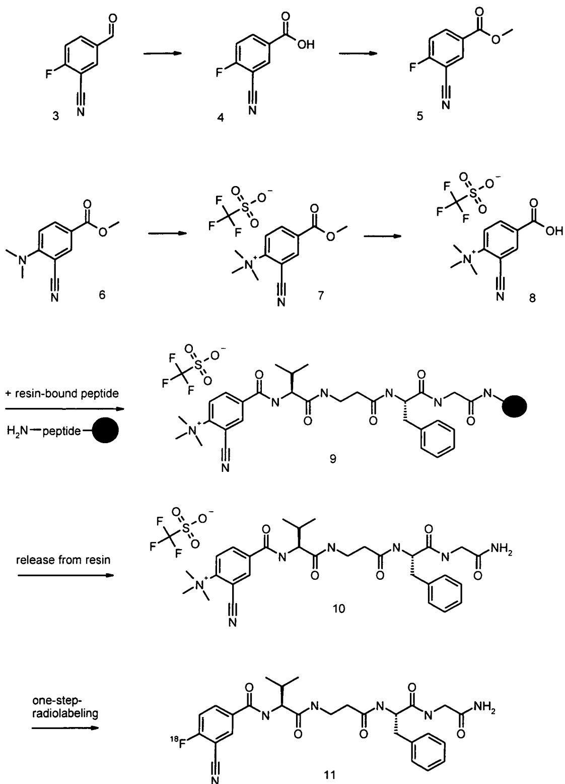
Scheme 3
