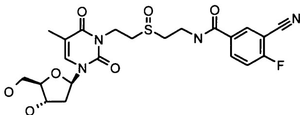
3-Cyano-4-fluoro-N-{2-[2-[3-((2R,4S,5R)-4-hydroxy-5-hydroxymethyl-tetrahydro-furan-2-yl)-5-methyl-2,6-dioxo-3,6-dihydro-2H-pyrimidin-1-yl]-ethanesulfonyl]-ethyl}-benzamide
