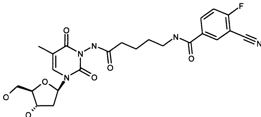
3-Cyano-4-fluoro-N-{4-[3-((2R,4S,5R)-4-hydroxy-5-hydroxymethyl-tetrahydro-furan-2-yl)-5-methyl-2,6-dioxo-3,6-dihydro-2H-pyrimidin-1-ylcarbonyl]-butyl}-benzamide
