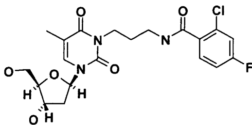
2-Chloro-4-fluoro-N-{3-[3-((2R,4S,5R)-4-hydroxy-5-hydroxymethyl-tetrahydro-furan-2-yl)-5-methyl-2,6-dioxo-3,6-dihydro-2H-pyrimidin-1-yl]-propyl}-benzamide
