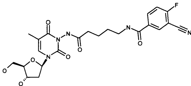
3-Cyano-4-fluoro-N-{4-[3-((2R,4S,5R)-4-hydroxy-5-hydroxymethyl-tetrahydro-furan-2-yl)-5-methyl-2,6-dioxo-3,6-dihydro-2H-pyrimidin-1-yl]-butyl}-benzamide
