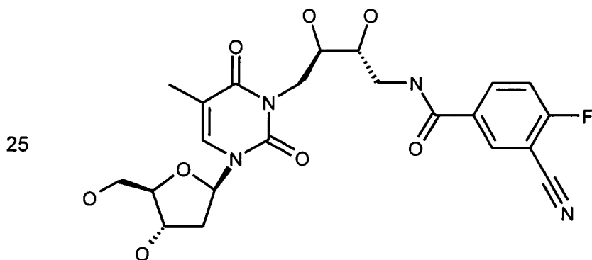
20 3-Cyano-4-fluoro-N-(2-{2-[3-((2R,4S,5R)-4-hydroxy-5-hydroxymethyl-tetrahydro-furan-2-yl)-5-methyl-2,6-dioxo-3,6-dihydro-2H-pyrimidin-1-yl]-ethylsulfanyl}-ethyl)-benzamide
