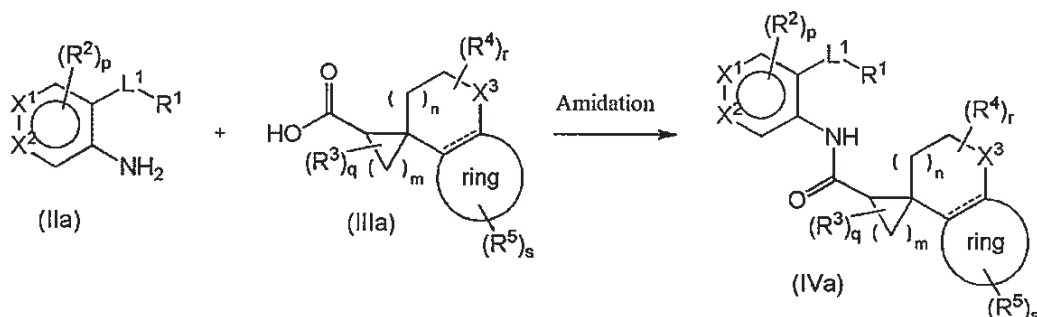
Reaction Scheme (Ia)
