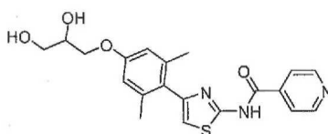
N -(4-(4-(2,3-Dihydroxypropoxy)-2,6-dimethylphenyl)thiazol-2-yl)isonicotinamide compound II-97
