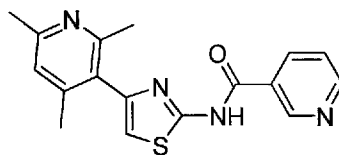
N -(4-(2,4,6-Trimethylpyridin-3-yl)thiazol-2-yl)nicotinamide compound II-46
