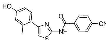
4-Cyano- N -(4-(4-hydroxy-2-methylphenyl)thiazol-2-yl)benzamide compound II-61
