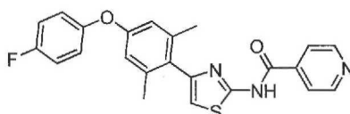
N -(4-(4-(4-Fluorophenoxy)-2,6-dimethylphenyl)thiazol-2-yl)isonicotinamide compound II-96
