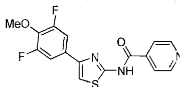
N -(4-(3,5-Difluoro-4-methoxyphenyl)thiazol-2-yl)isonicotinamide compound II-62
