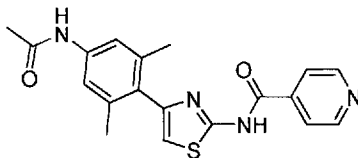
N -(4-(4-Acetamido-2,6-dimethylphenyl)thiazol-2-yl)isonicotinamide compound II-74
