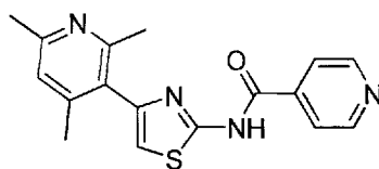
N -(4-(2,4,6-Trimethylpyridin-3-yl)thiazol-2-yl)isonicotinamide compound II-44
