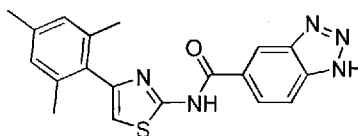
N -(4-Mesitylthiazol-2-yl)-1 H -benzo[ d ][1,2,3]triazole-5-carboxamide compound II-106
