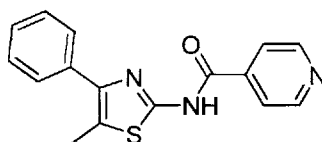
N -(5-Methyl-4-phenylthiazol-2-yl)isonicotinamide compound II-2
