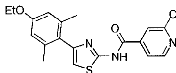
2-Chloro-N-(4-(4-ethoxy-2,6-dimethylphenyl)thiazol-2-yl)isonicotinamide compound II-66
