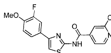
2-Chloro- N -(4-(3-fluoro-4-methoxyphenyl)thiazol-2-yl)isonicotinamide compound II-63
