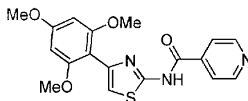
N -(4-(2,4,6-Trimethoxyphenyl)thiazol-2-yl)isonicotinamide compound II-11
