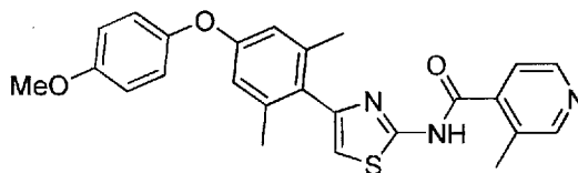
N-(4-(4-(4-Methoxyphenoxy)-2,6-dimethylphenyl)thiazol-2-yl)-3-methylisonicotinamide compound II-121
