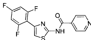
N -(4-(2,4,6-Trifluorophenyl)thiazol-2-yl)isonicotinamide compound II-76
