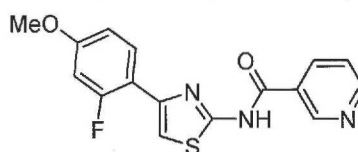
N -(4-(2-Fluoro-4-methoxyphenyl)thiazol-2-yl)nicotinamide compound II-21
