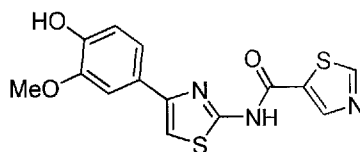
N -(4-(4-Hydroxy-3-methoxyphenyl)thiazol-2-yl)thiazole-5-carboxamide compound II-50
