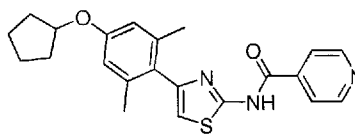
N -(4-(4-(Cyclopentyloxy)-2,6-dimethylphenyl)thiazol-2-yl)isonicotinamide compound II-85
