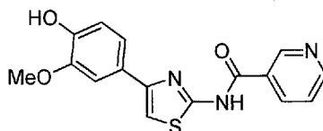
N -(4-(4-Hydroxy-3-methoxyphenyl)thiazol-2-yl)nicotinamide compound II-35
