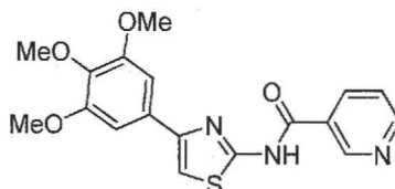
N -(4-(3,4,5-Trimethoxyphenyl)thiazol-2-yl)nicotinamide compound II-20
