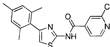
2-Chloro-N-(4-mesitylthiazol-2-yl)isonicotinamide compound II-64
