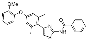
N -(4-(4-(2-Methoxyphenoxy)-2,6-dimethylphenyl)thiazol-2-yl)isonicotinamide compound II-111
