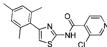
3-Chloro-N-(4-mesitylthiazol-2-yl)isonicotinamide compound II-80
