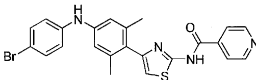
N-(4-(4-(4-Bromophenylamino)-2,6-dimethylphenyl)thiazol-2-yl)isonicotinamide compound II-122
