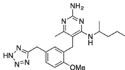
5-(5-((2 H -tetrazol-5-yl)methyl)-2-methoxybenzyl)-6-methyl- N 4 -(pentan-2-yl)pyrimidine-2,4-diamine
