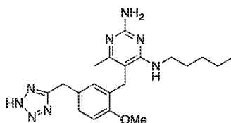
5-(5-((2H-tetrazol-5-yl)methyl)-2-methoxybenzyl)-6-methyl-N 4 -pentylpyrimidine-2,4-diamine Chemical Formula: C 20 H 28 N 8 O Exact Mass: 396.24
