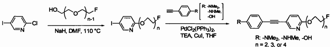
SCHEME 13
