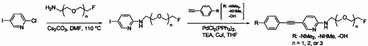
SCHEME 15
