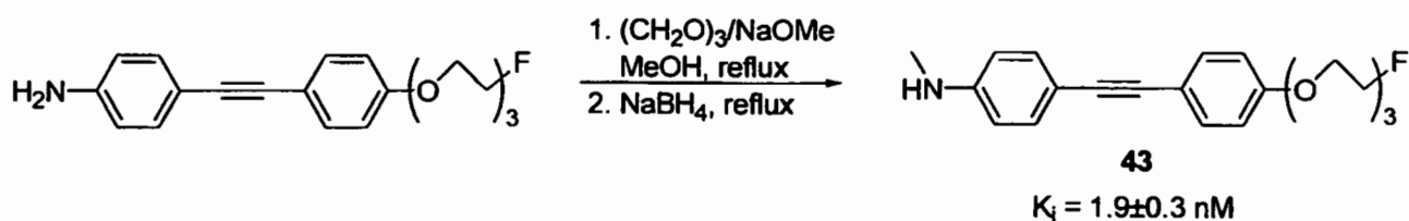
SCHEME 11
