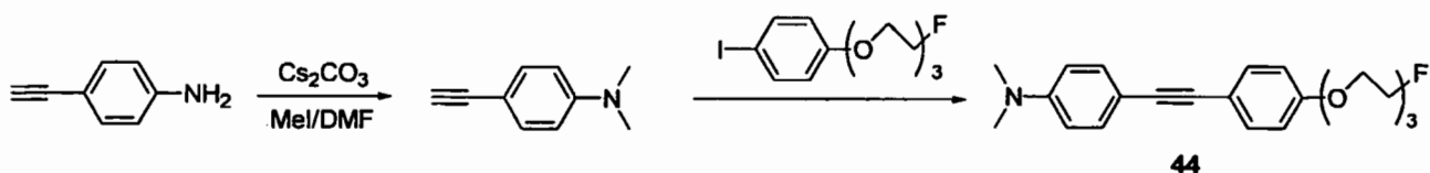
SCHEME 11
