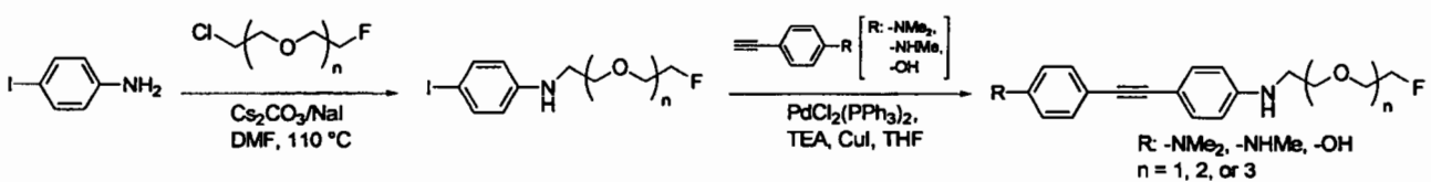
SCHEME 14
