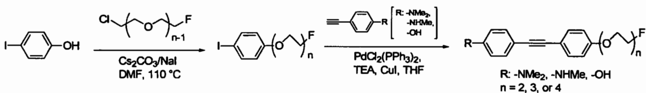
SCHEME 12
