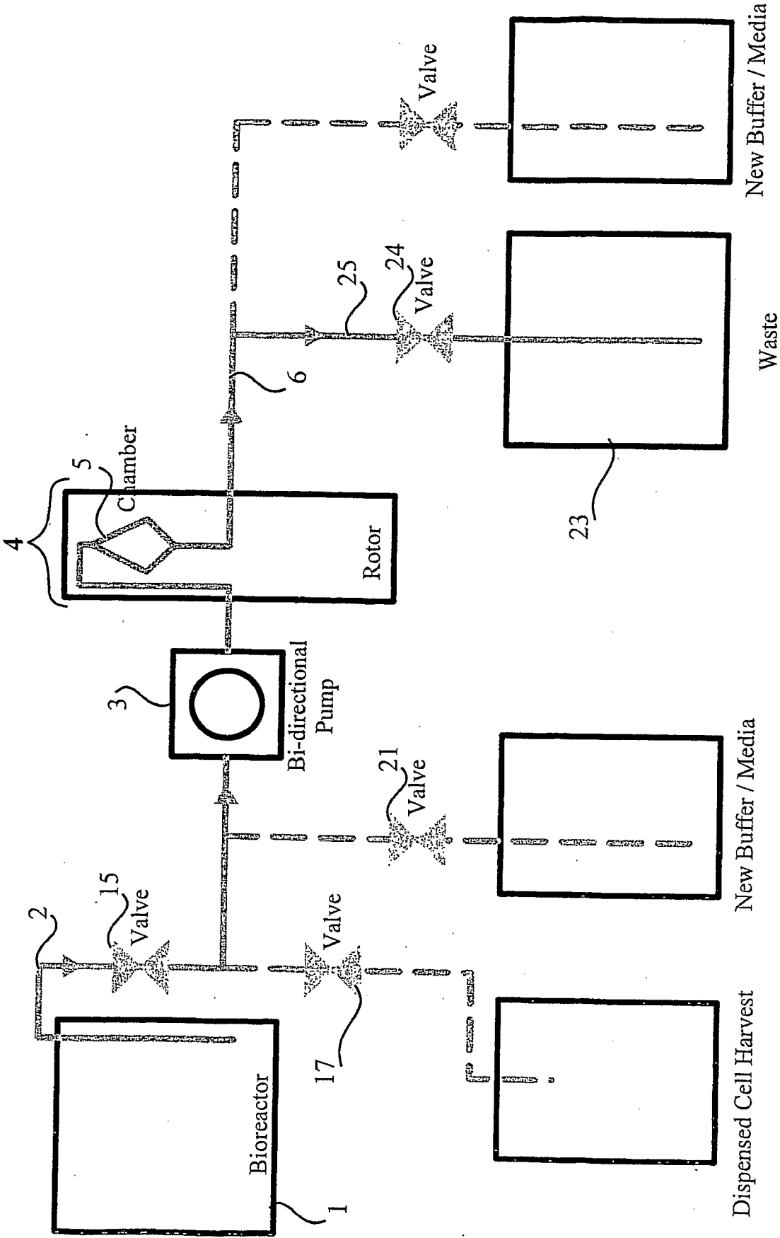
Figure 21 Cell Dispenser Flow Diagram Cell Capture Mode
