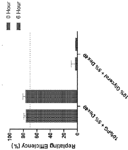
Replating Efficiency
