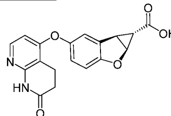
Intermediate 8
