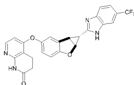
Compound 1
