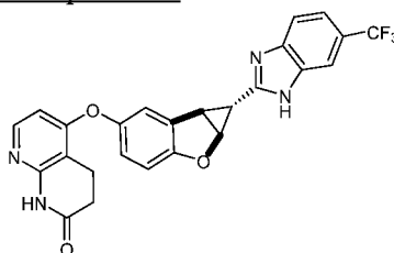
free base of Compound 1
