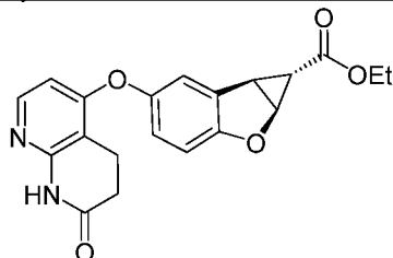
Intermediate 7
