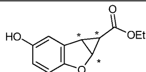
Intermediate 5
