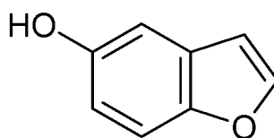
Intermediate 1
