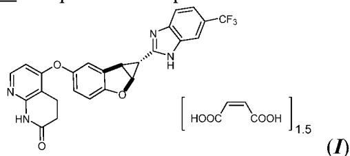
Compound 1 Sesqui-Maleate
