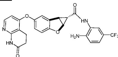
Intermediate 9
