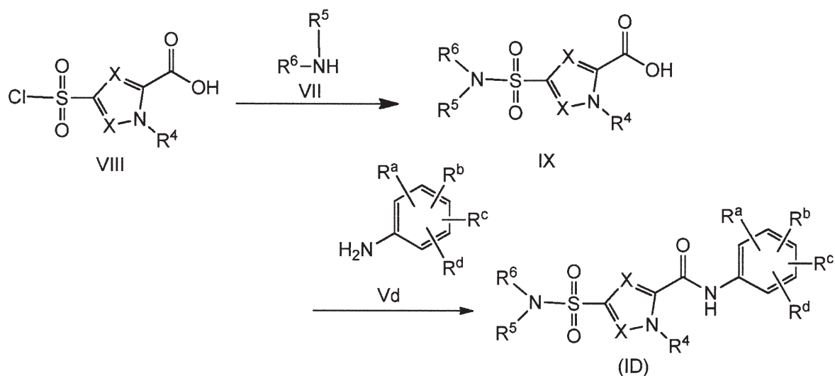
Scheme 2b
