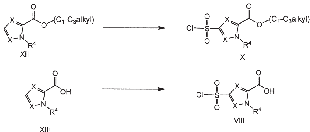
Scheme 4
