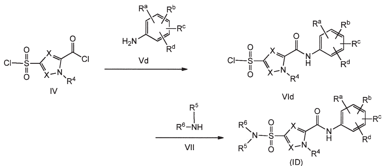
Scheme 1b
