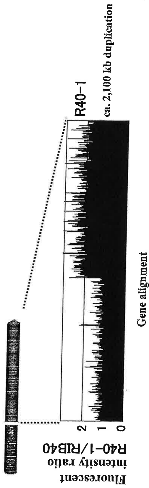
Fig. 9 Second chromosome
