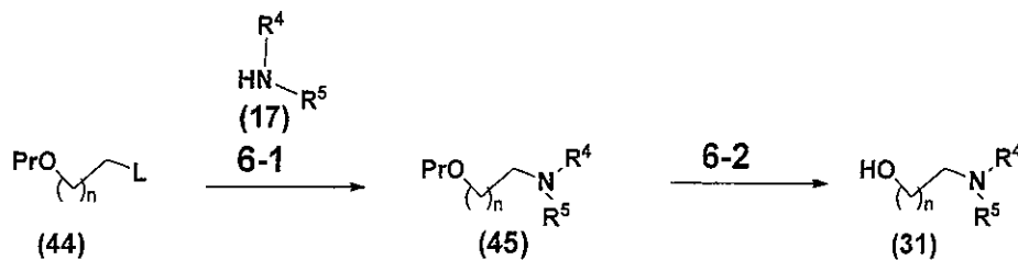
Scheme 6
