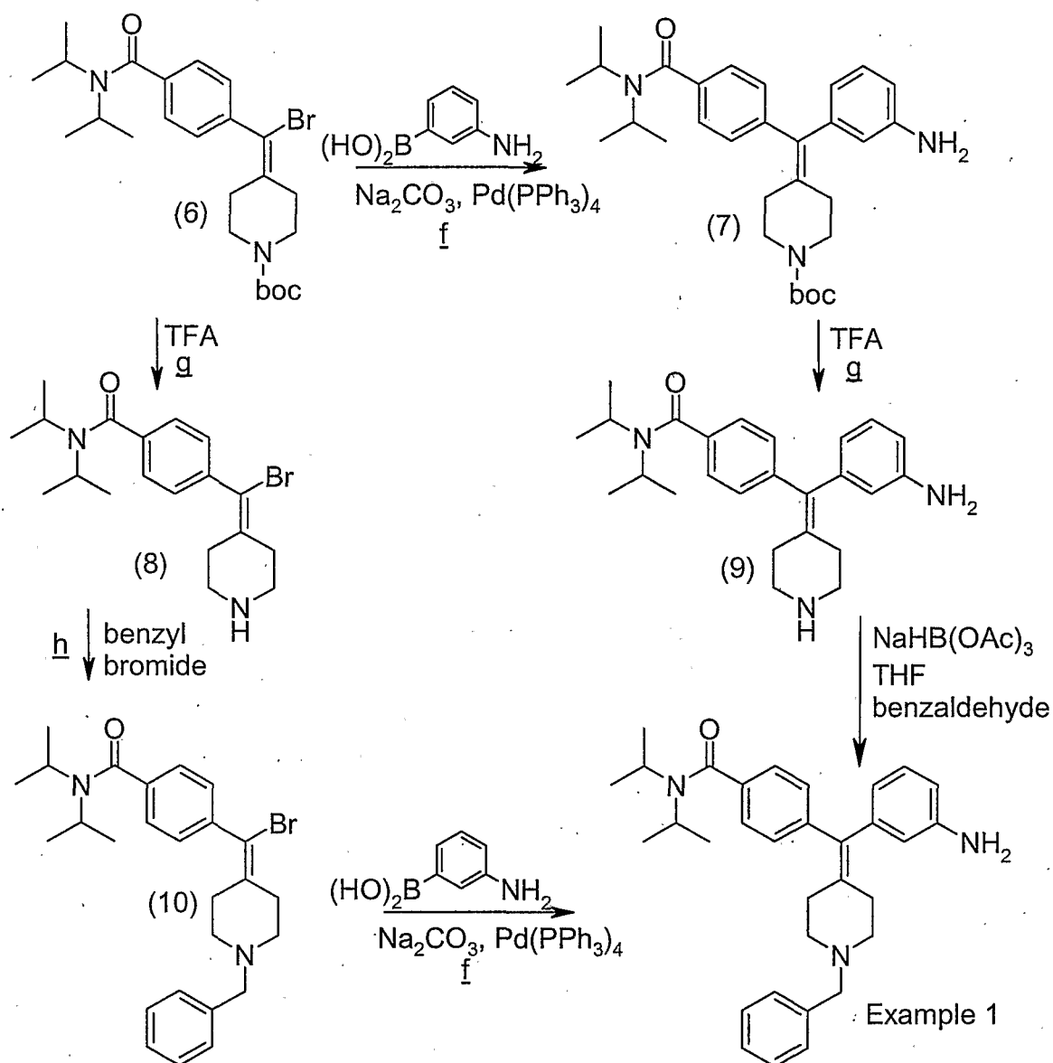
Scheme 2: Synthetic route to Example 1 and Intermediate 9
