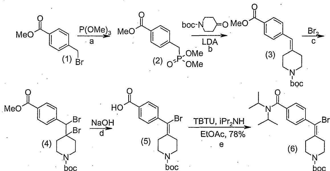
Scheme 1: Synthesis of vinyl bromide intermediate 6.
