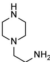
Aminoethylpiperazine (AEP)
