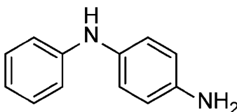
N-phenyl-p-phenylenediamine (NPPDA)
