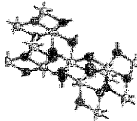
Anatase
