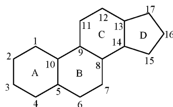
Formula I: Steroidal Backbone
