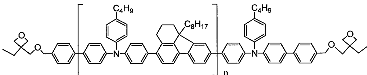
Compound 5
