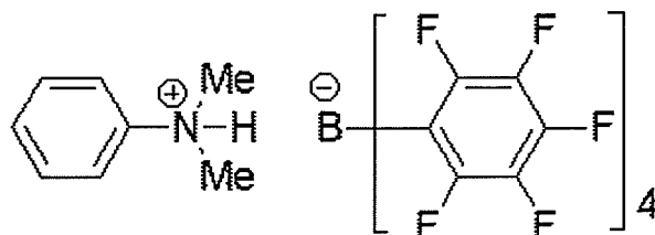
Polymerization initiator
