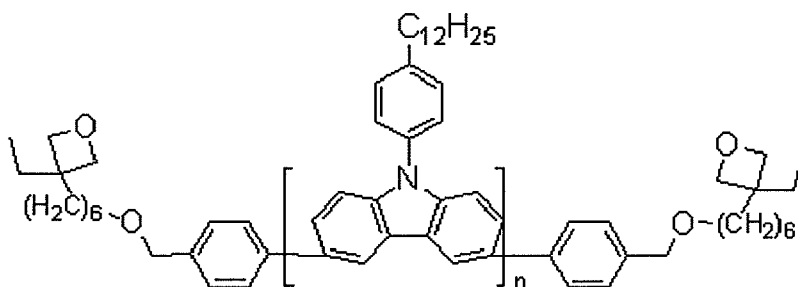
Compound 3
