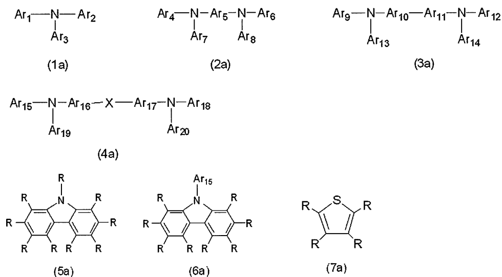
[Chemical Formula 1]
