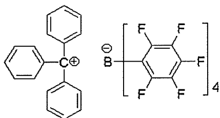
Ionic compound 1
