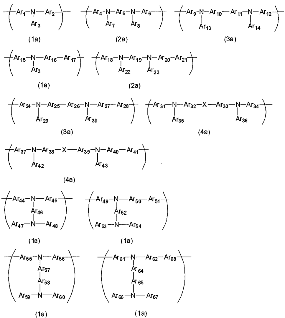
[Chemical Formula 3]
