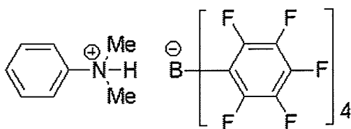
Ionic compound 2
