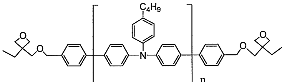
Compound 4
