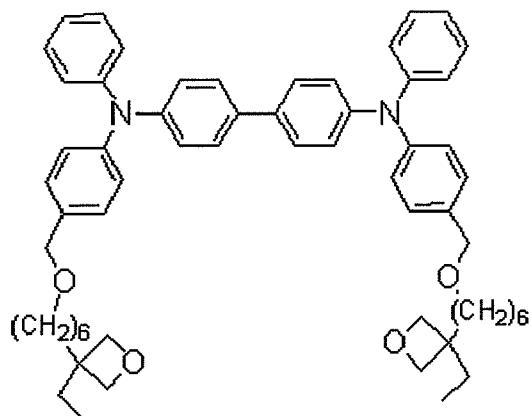
Compound 1
