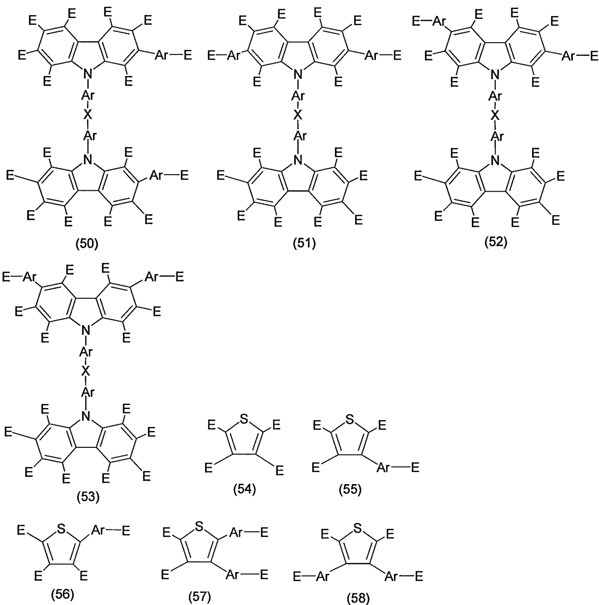
[Chemical Formula 11]
