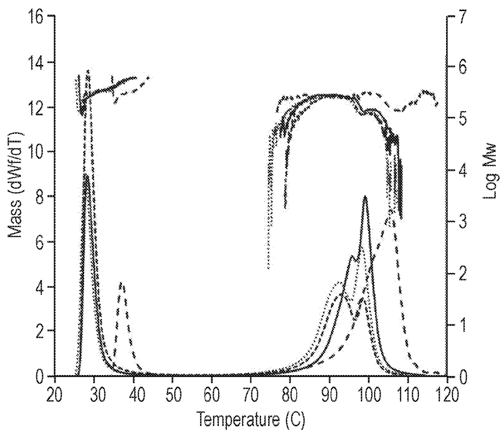
FIG. 3 CEF Overlay Polymerization Examples
