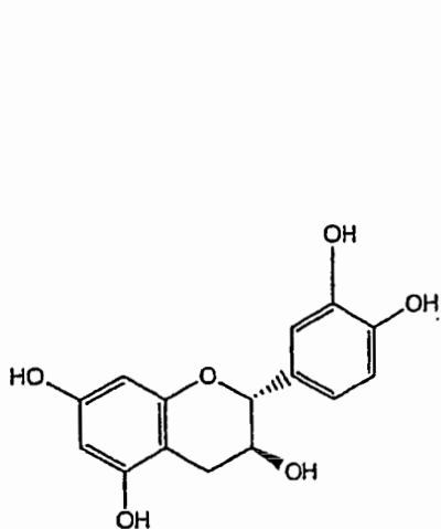
Catechin
