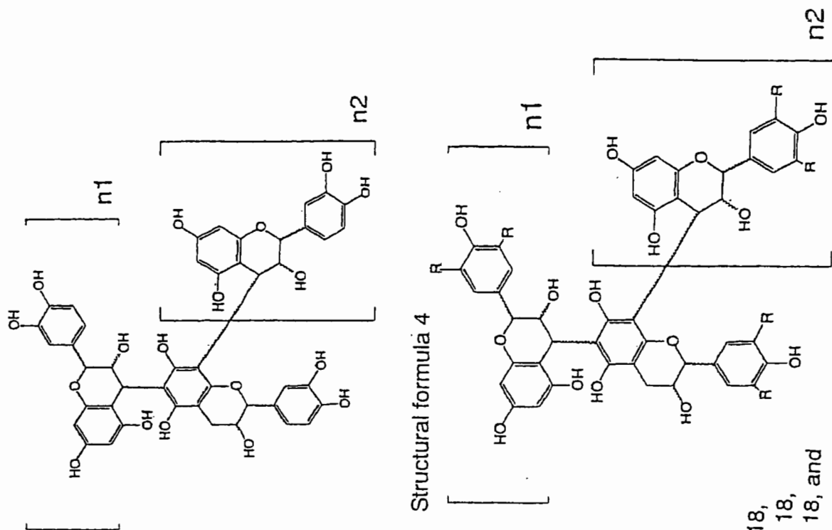
Structural formula 2
