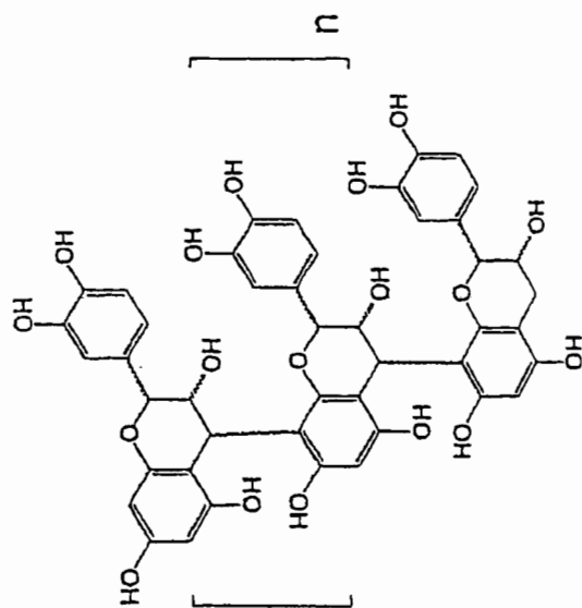
Structural formula 1
