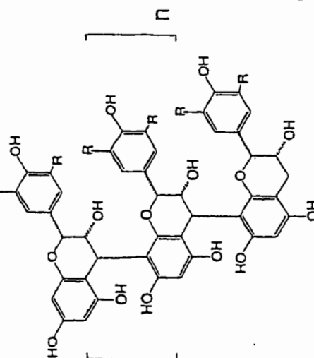
Structural formula 3
