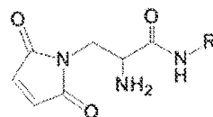
\beta -maleimido DPR
