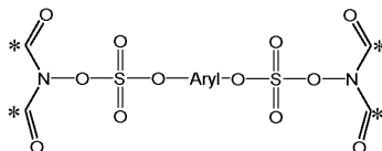
N-(carbonylcarbamido) aryl sulfate with a second N-(carbonylcarbamido) aryl sulfate moiety
