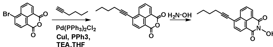
Scheme 3 Synthetic pathway for N-hydroxy-4-(hex-1-yn-1-yl)-1,8-naphthalimide.
