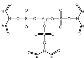
N-(carbonylcarbamido) aryl sulfate with a third N-(carbonylcarbamido) sulfate moiety
