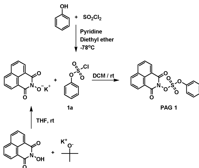
Scheme 1 Synthesis of PAG 1
