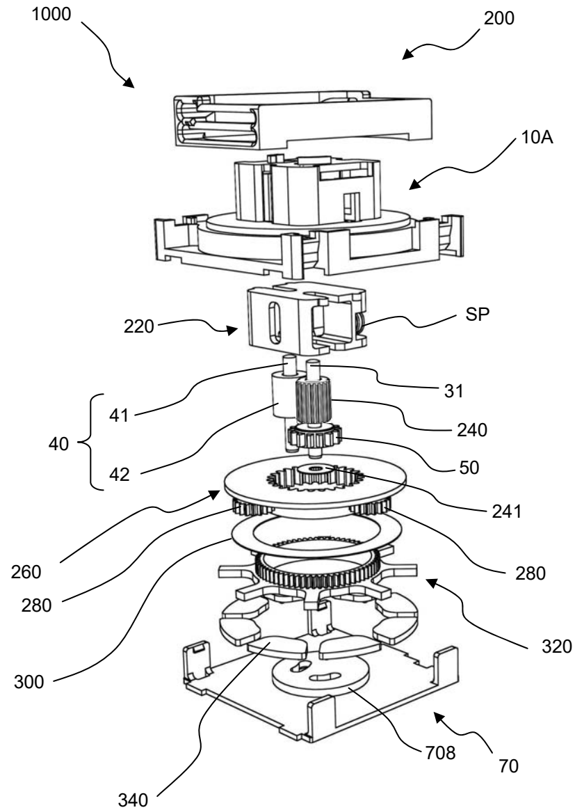
Fig. 11A EXPLODED PERSPECTIVE VIEW SEEN FROM FRONT-UPPER SIDE
