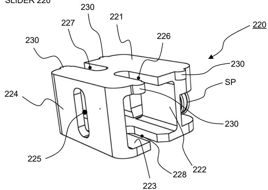
Fig. 23A FRONT PERSPECTIVE VIEW
