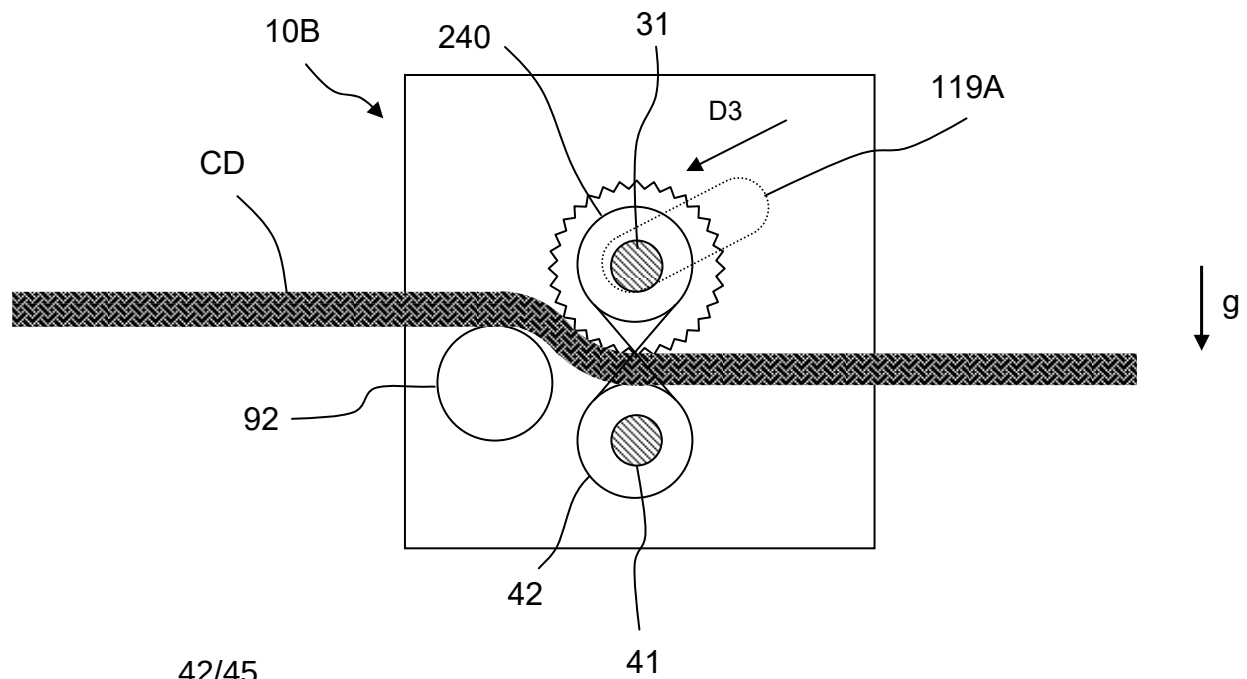
Fig. 40B SANDWICHED STATE
