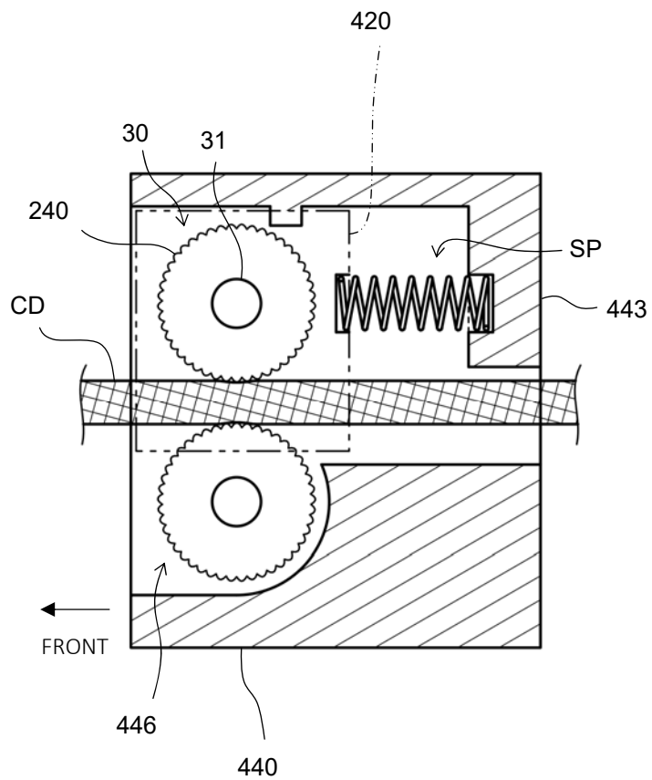
Fig. 36A OUTPUT STATE
