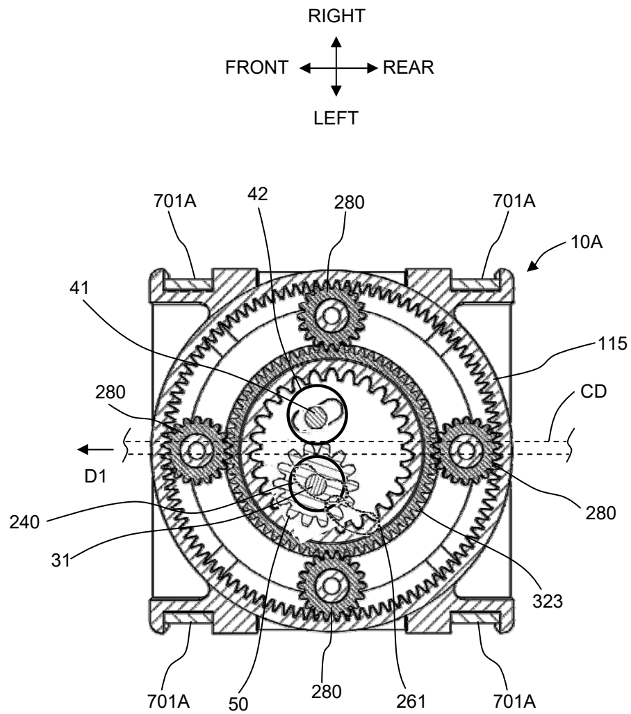
Fig. 28A STEADY STATE
