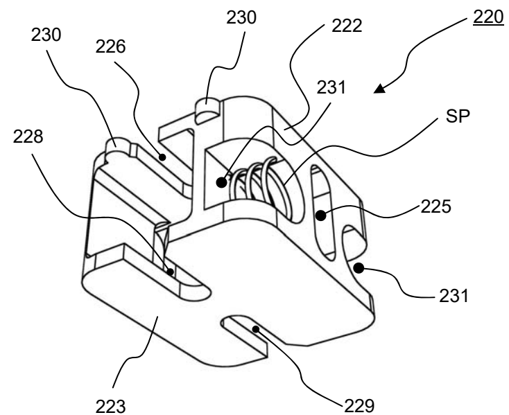
Fig. 23B REAR PERSPECTIVE VIEW
