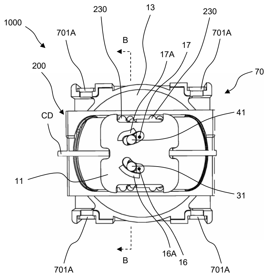
Fig. 15A PLAN VIEW
