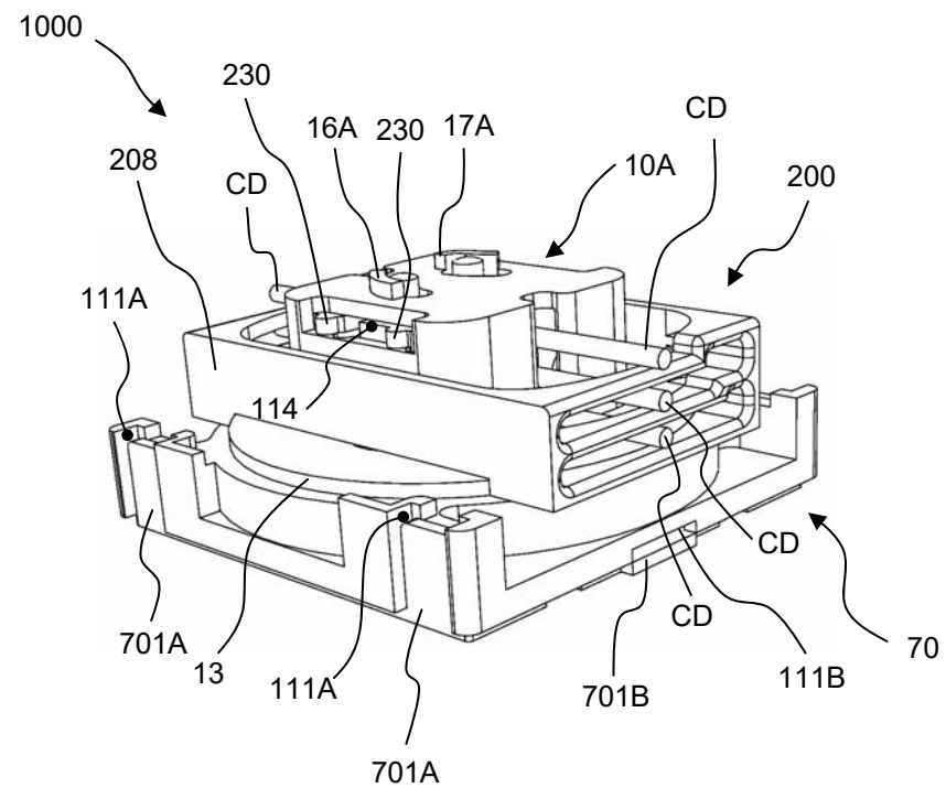
Fig. 14B REAR PERSPECTIVE VIEW
