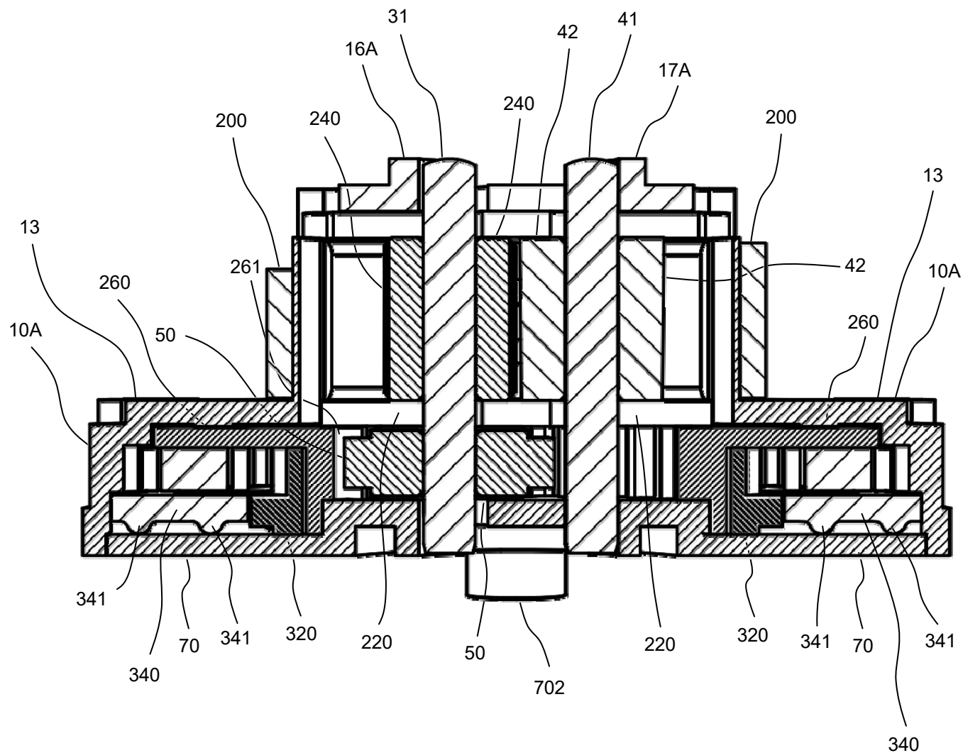
LINE B-B SECTIONAL VIEW
