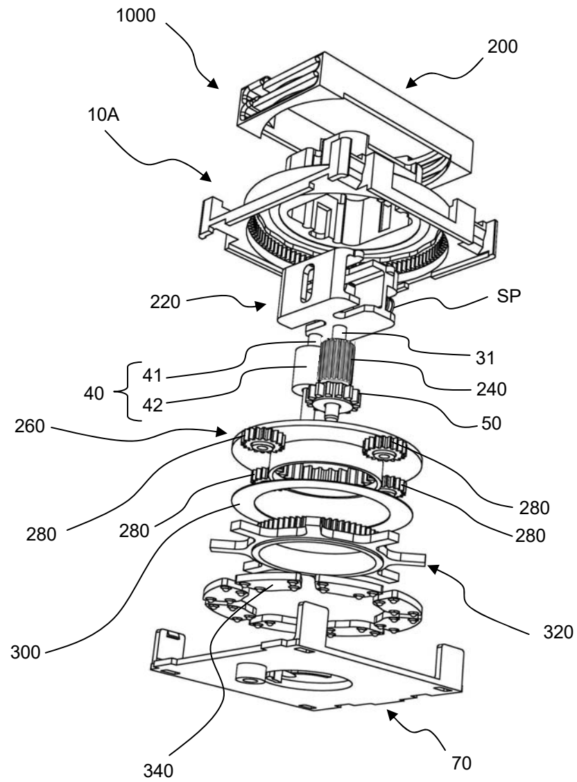
Fig. 12A EXPLODED PERSPECTIVE VIEW SEEN FROM FRONT-LOWER SIDE
