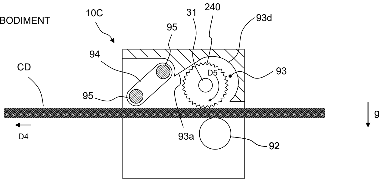
Fig. 41A FREE MOVEMENT STATE
