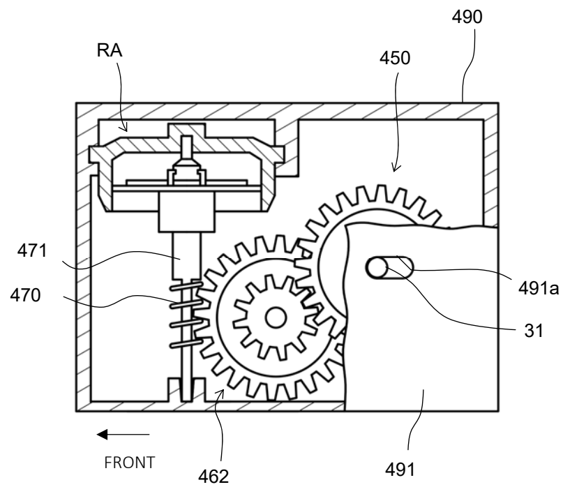
Fig. 35A OUTPUT STATE
