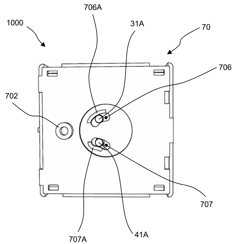
Fig. 15B BOTTOM VIEW
