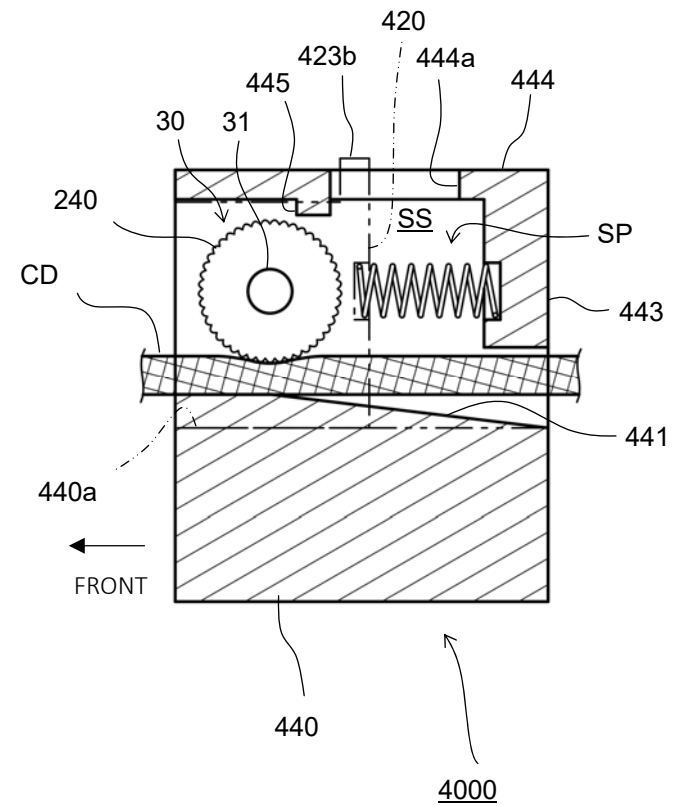
Fig. 32B LINE E-E END VIEW
