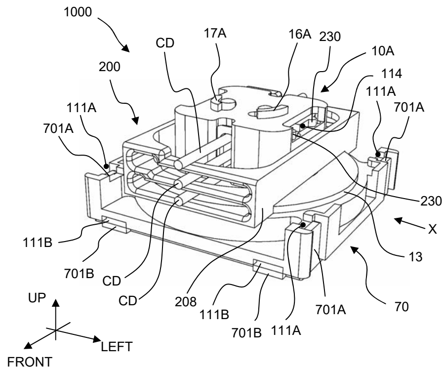
Fig. 14A FRONT PERSPECTIVE VIEW
