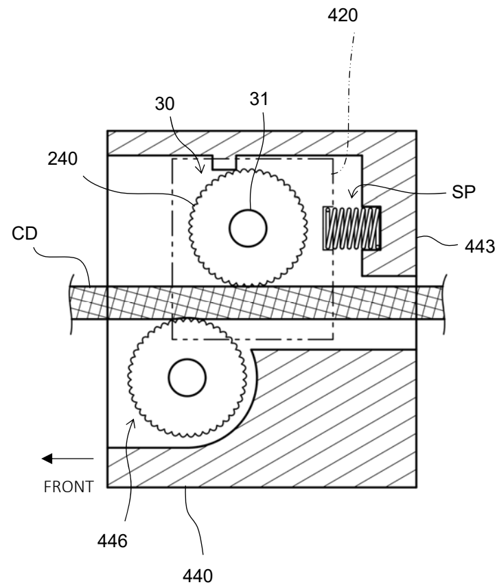
Fig. 36B RELEASE STATE
