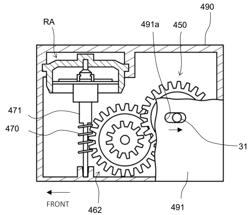
Fig. 35B RELEASE STATE
