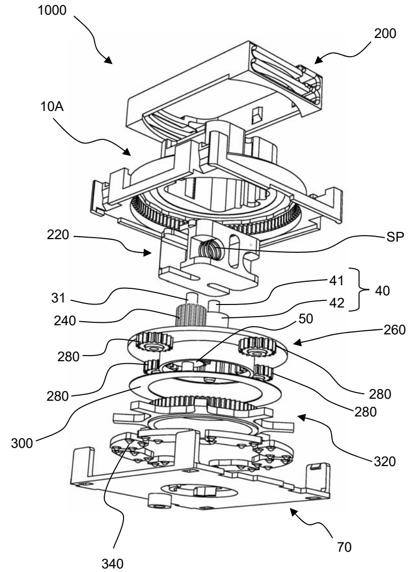
Fig. 12B EXPLODED PERSPECTIVE VIEW SEEN FROM REAR-LOWER SIDE
