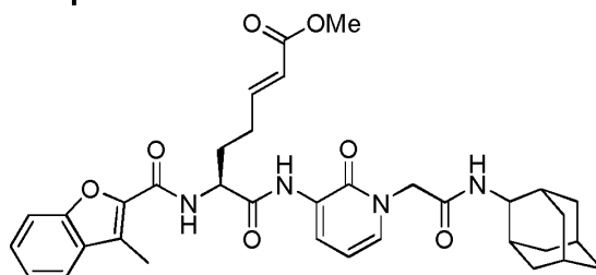
( S,E )-methyl 7-(1-(2-(2-adamantylamino)-2-oxoethyl)-2-oxo-1,2-dihydropyridin-3-ylamino)-6-(3-methylbenzofuran-2-carboxamido)-7-oxohept-2-enoate Chemical Formula: C 35 H 40 N 4 O 7 Exact Mass: 628.29 Molecular Weight: 628.71
