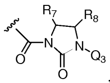
Formula IV
