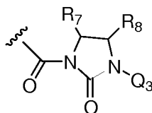
Formula IV
