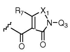
Formula V
