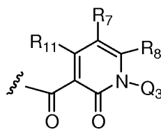
Formula VII
