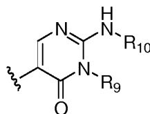
Formula II
