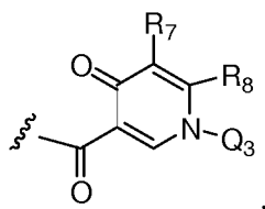
Formula VI
