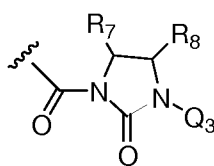
Formula IV
