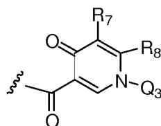
Formula VI
