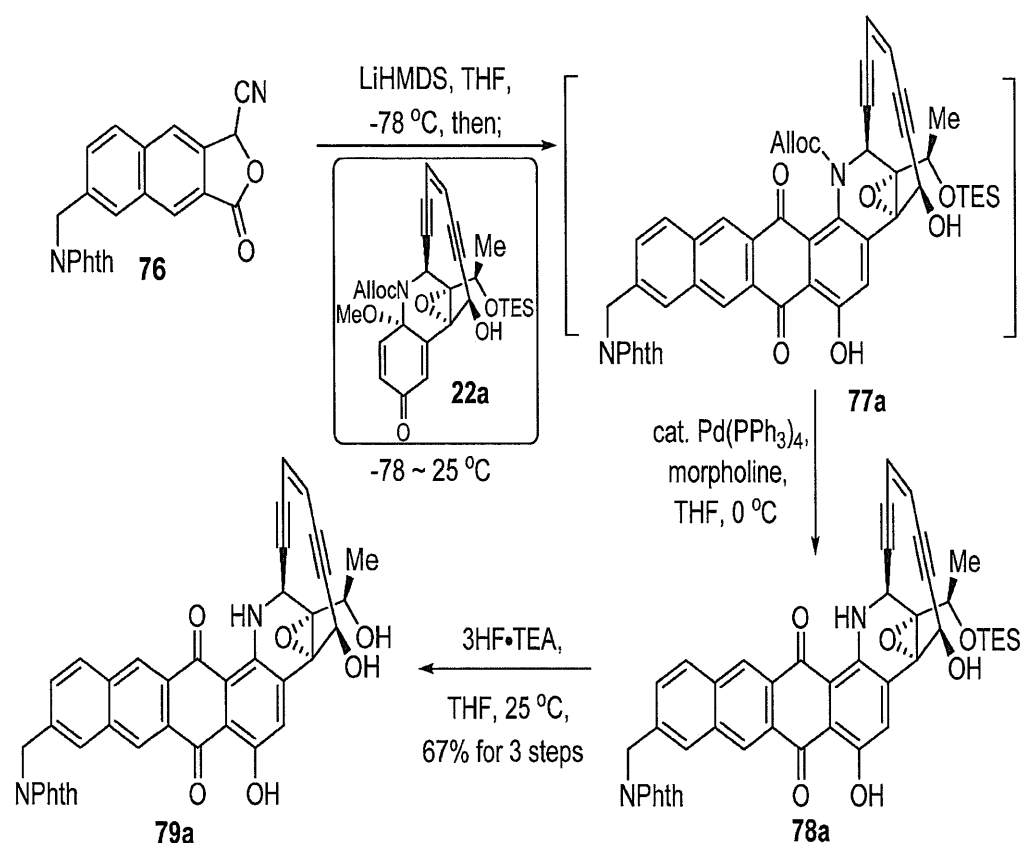
Scheme 14. Synthesis of phthalimidomethyl-benzo-uncialamycins 79a .
