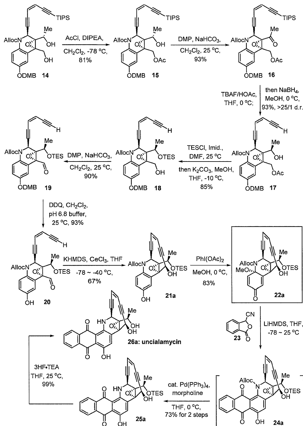
Scheme 3. Improved synthesis of unciamycin (26a). Construction of key intermediate 22a and completion of the synthesis.
