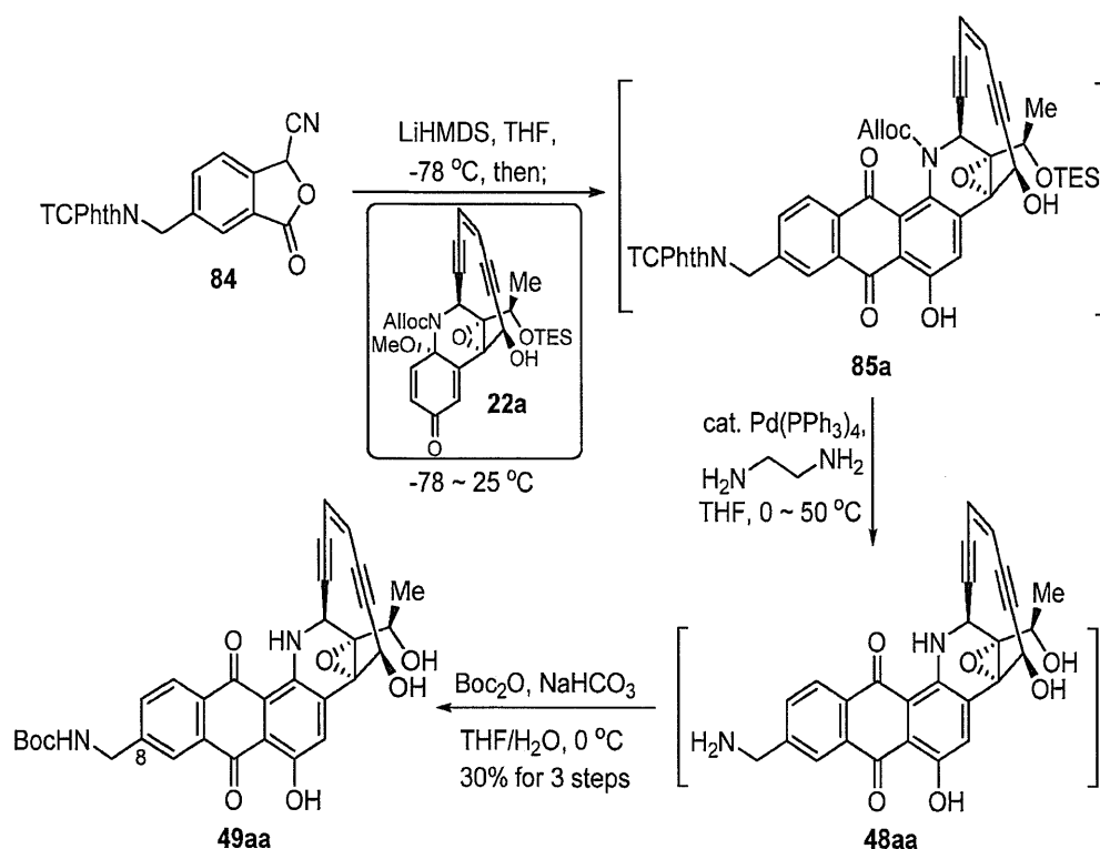
Scheme 16. Synthesis of 8-aminomethyl-uncialamycin 48aa and 49aa .
