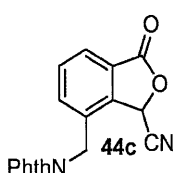
Scheme 6. Synthesis of cyanophthalides 44a , 44b , 44c , and 44d .
