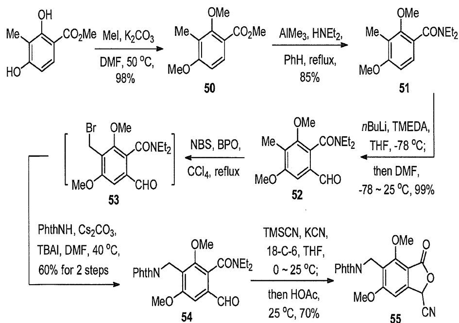
Scheme 9. Synthesis of cyanophthalides 55 .
