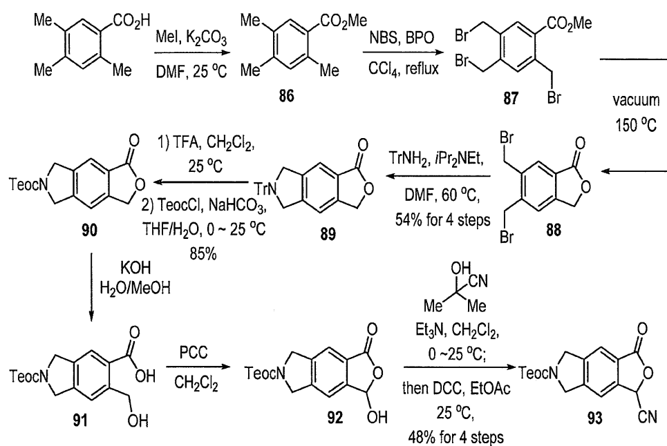
Scheme 17. Synthesis of cyanophthalide 93.
