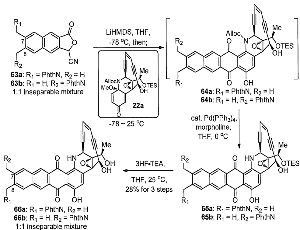
Scheme 12. Synthesis of 8-phthalimidomethyl-uncialamycins 66a/66b .
