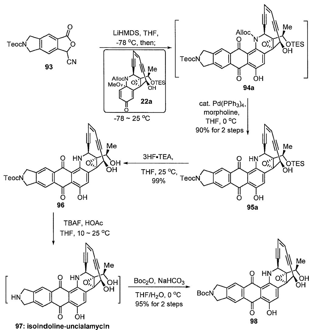
Scheme 18. Synthesis of isoindoline-uncialamycins ( 96 , 97 , and 98 ).
