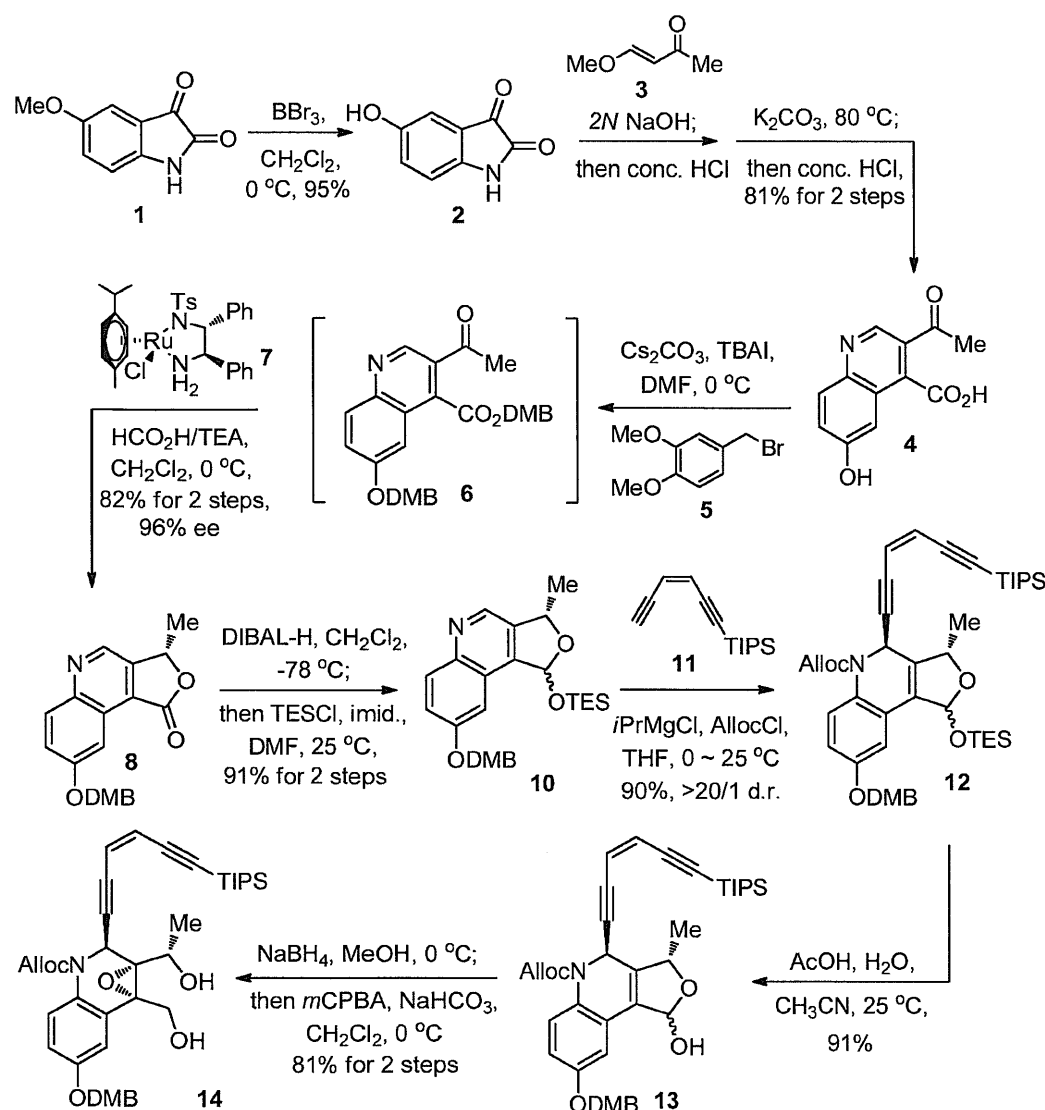
Scheme 2. Improved synthesis of unciamycin ( 26a ). Construction of key intermediate 14 .
