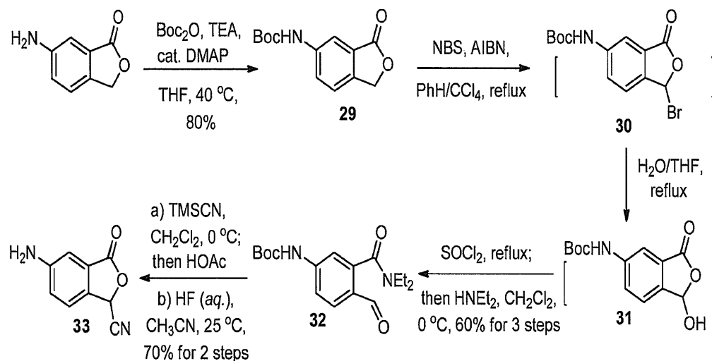
Scheme 4. Synthesis of cyanophthalide 33 .
