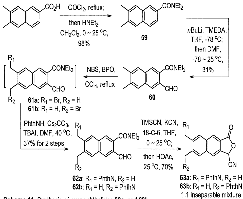
Scheme 11. Synthesis of cyanophthalides 63a , and 63b .
