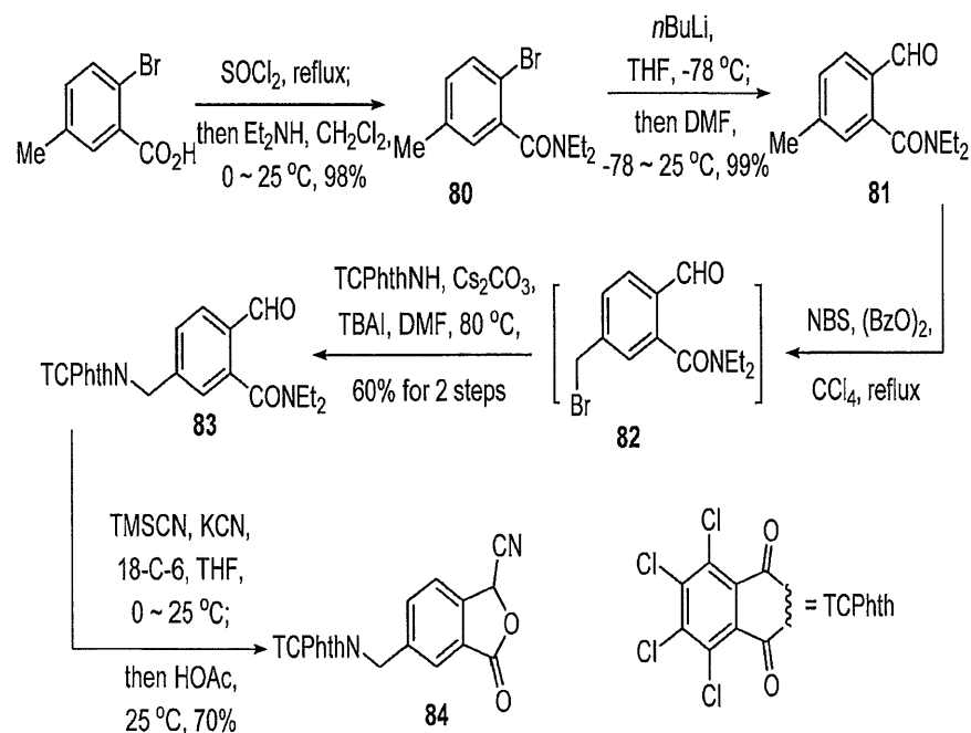
Scheme 15. Synthesis of cyanophthalides 84 .
