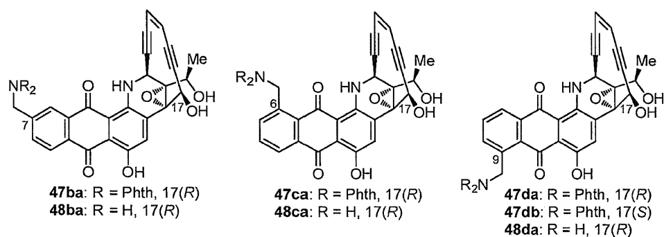
Scheme 7. Synthesis of aminomethyl-uncialamycins (48aa, 48ba, 48ca, and 48da).
