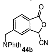
Scheme 6. Synthesis of cyanophthalides 44a , 44b , 44c , and 44d .
