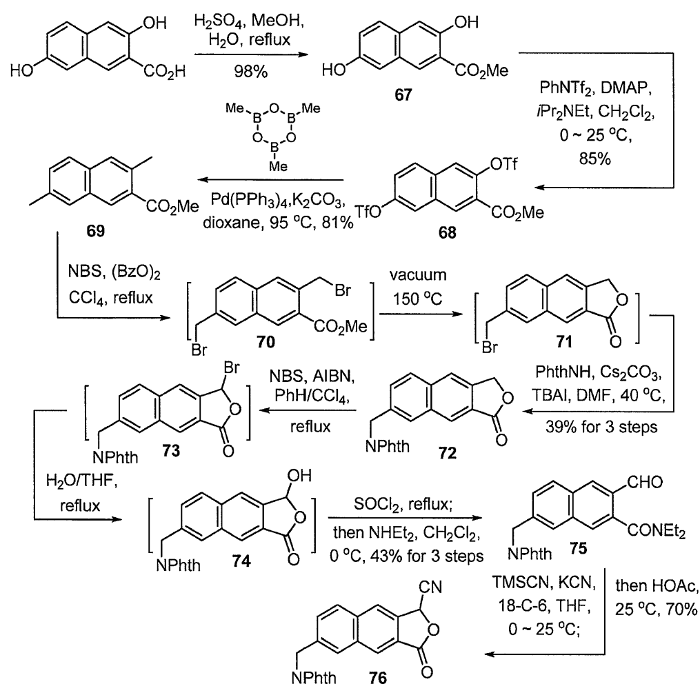
Scheme 13. Synthesis of cyanophthalide 76 .
