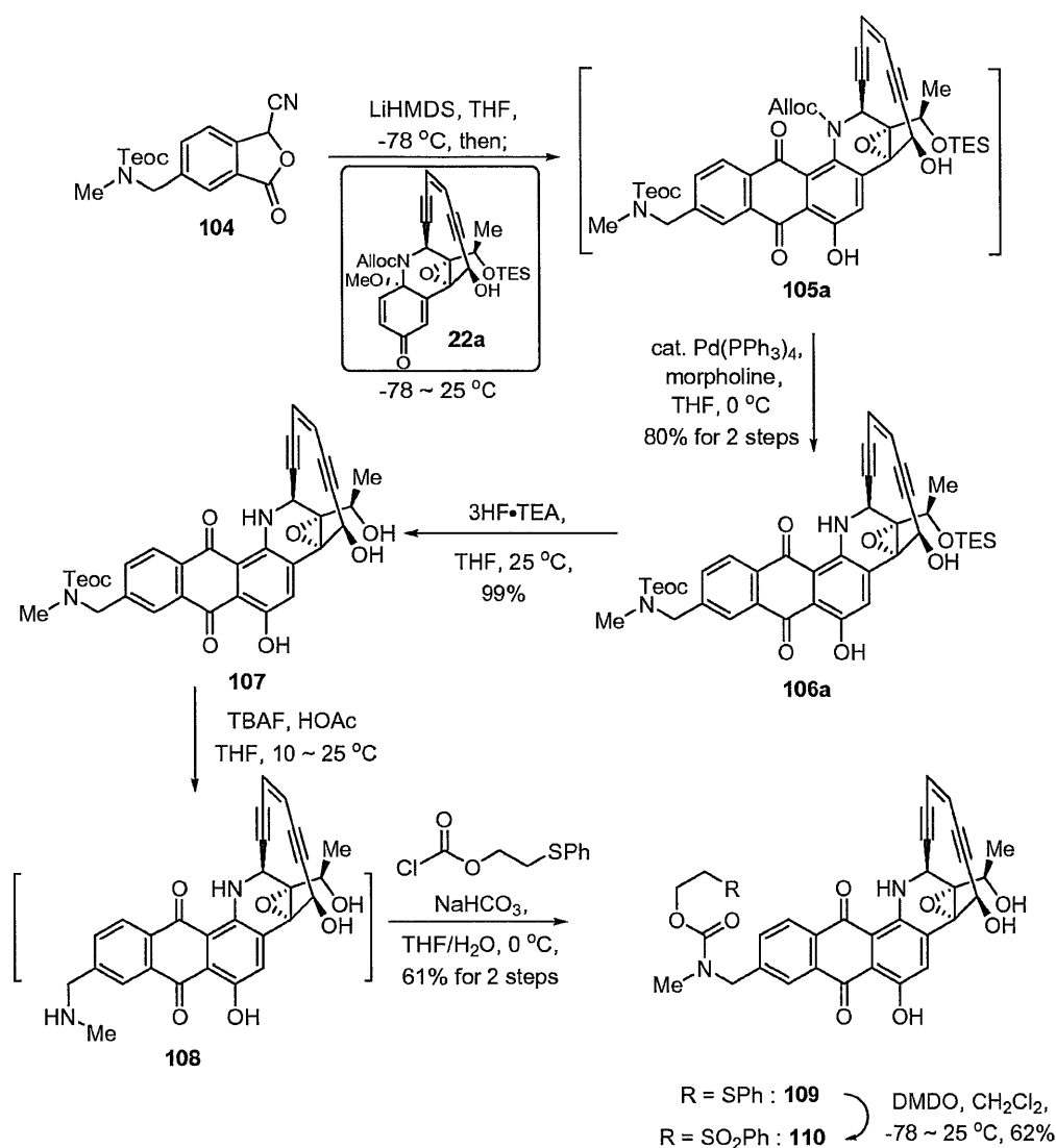
Scheme 21. Synthesis of 8-N-methylaminomethyl-uncialamycins ( 107 , 108 , 109 , and 110 ).
