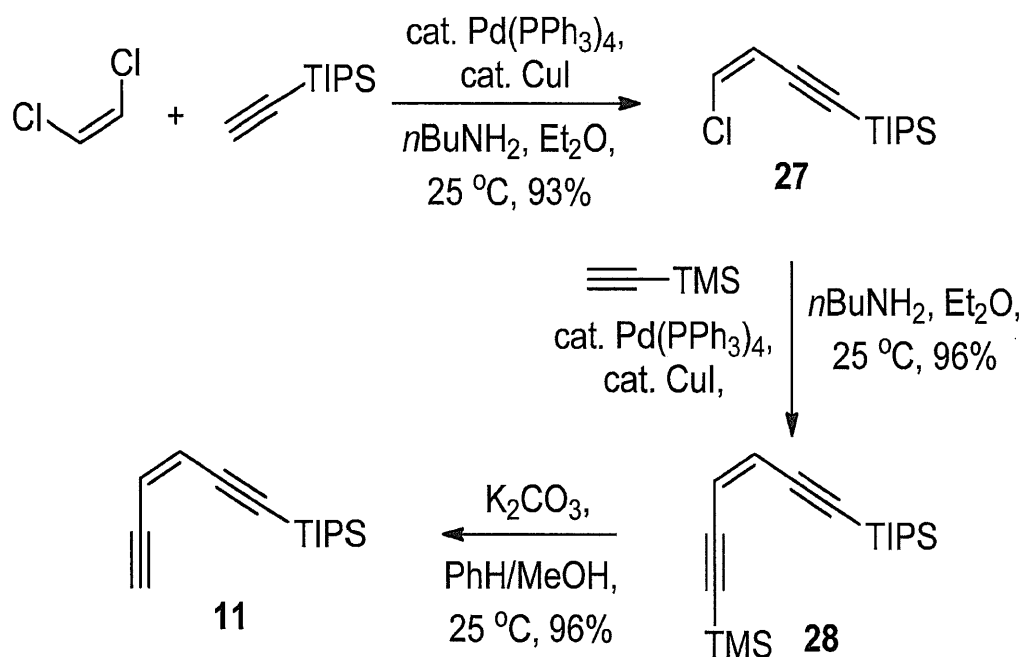
Scheme 1. Synthesis of enediyne building block 11 .
