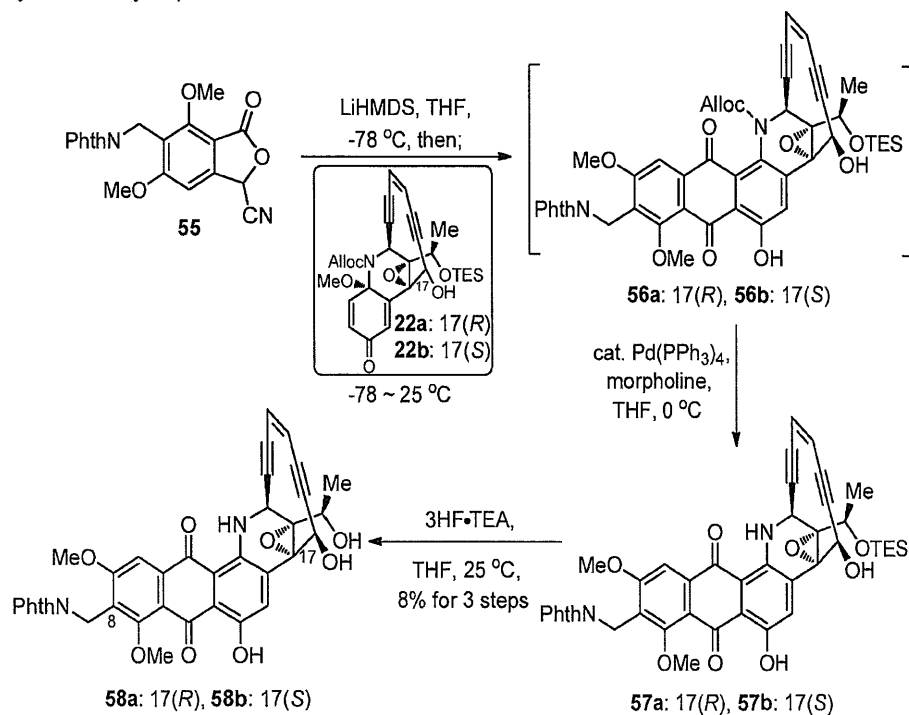
Scheme 10. Synthesis of 8-phthalimidomethyl-unciamycin 58a , and 58b .
