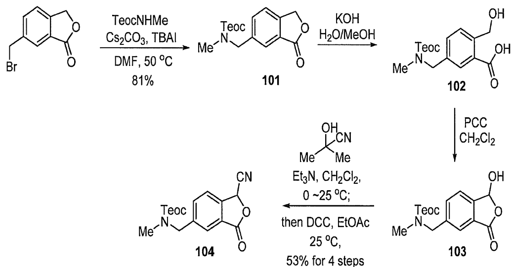
Scheme 20. Synthesis of cyanophthalide 104 .
