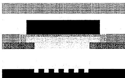
(i) Aluminum Reflecting layer deposited
