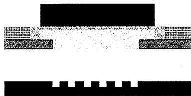
(g) Porous Gold Black evaporation and patterning
