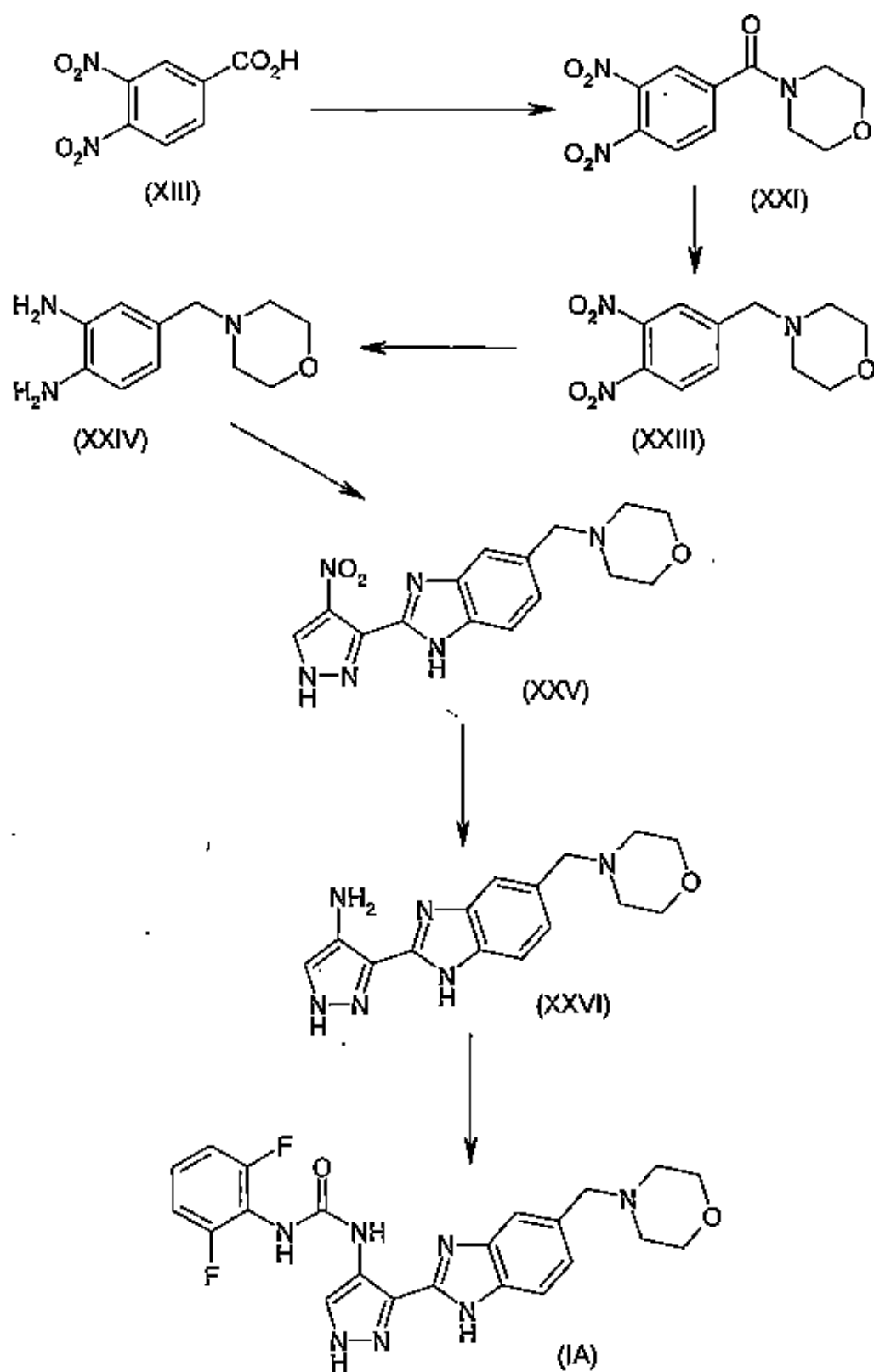
Scheme 3
