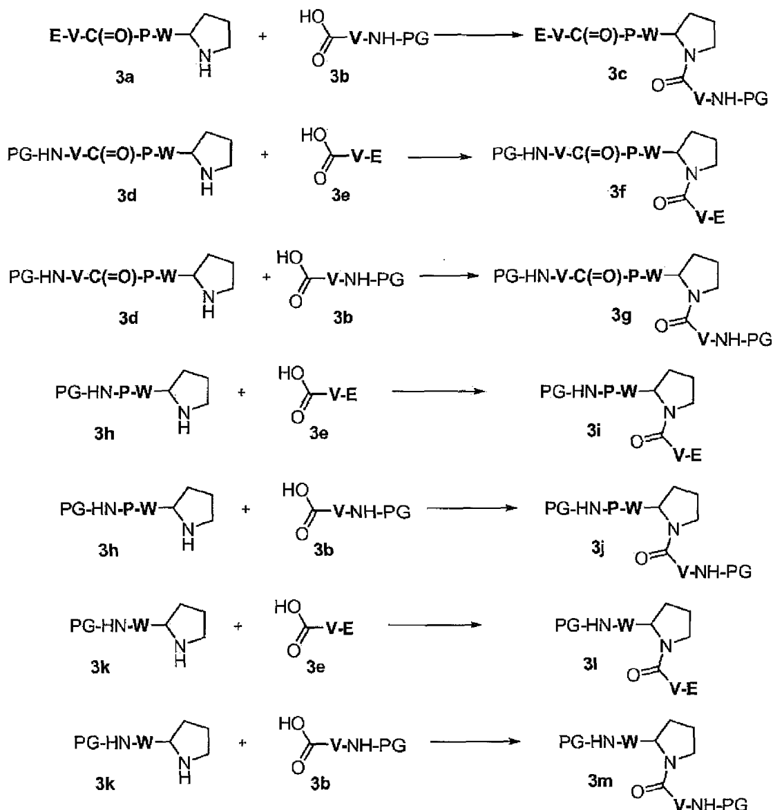
Scheme 3. Representative synthesis of R^1-V-C(=O)-P-R^2
