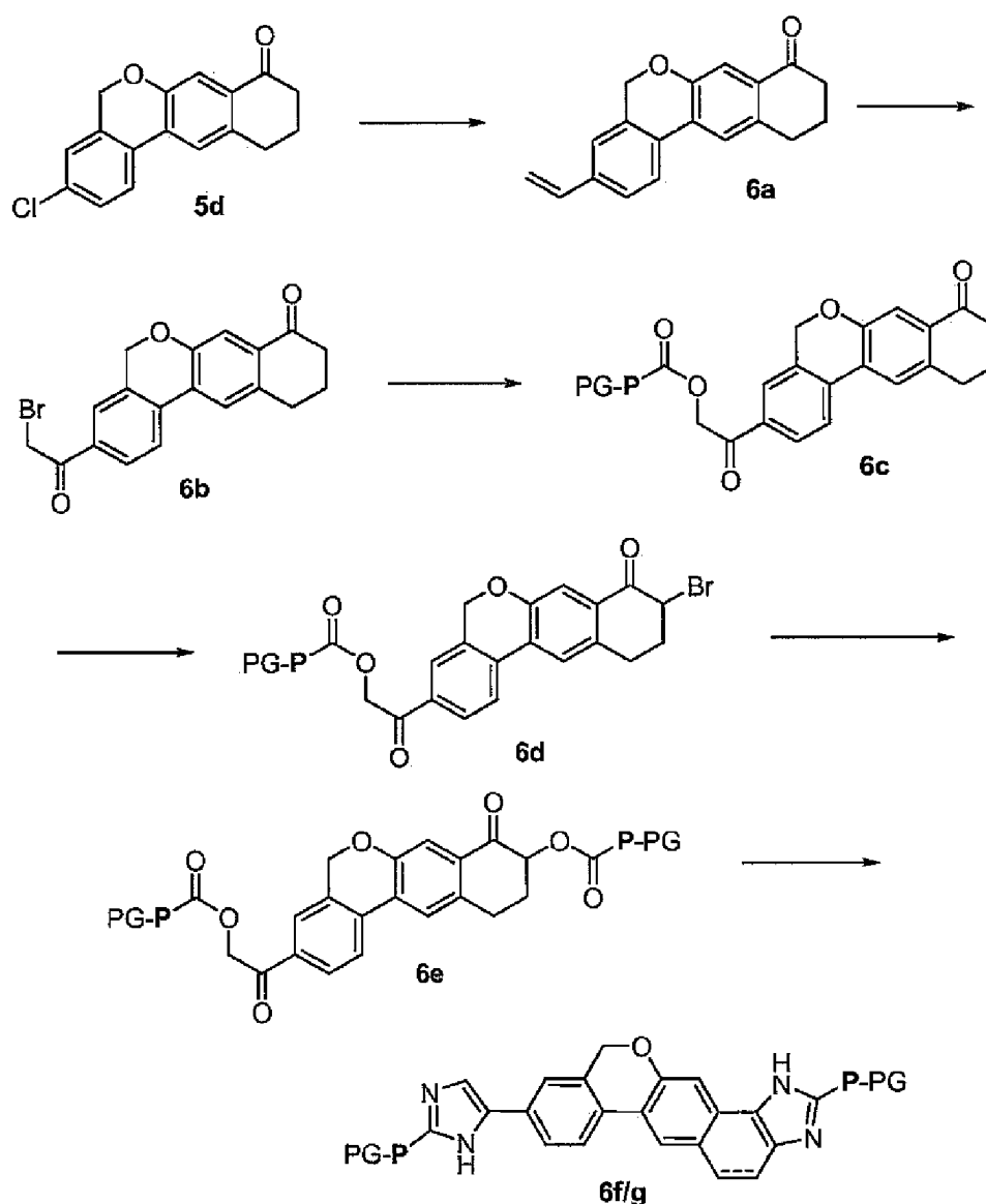
Scheme 6. Representative synthesis of \text{R}^1\text{-P-W-P-R}^2
