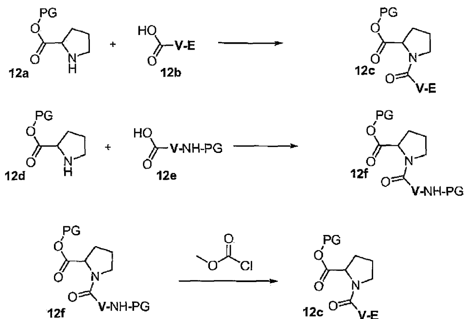
Scheme 12. Representative synthesis of R^1-V-C(=O)-P-R^2
