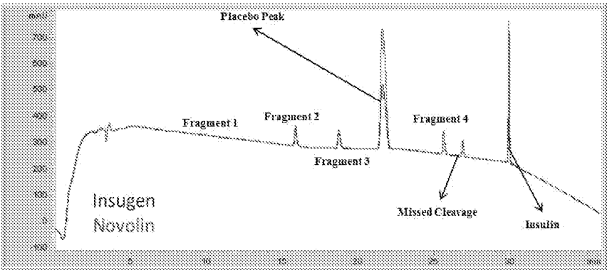
Figure 5: Overlays of Insulin samples under digestion conditions.
