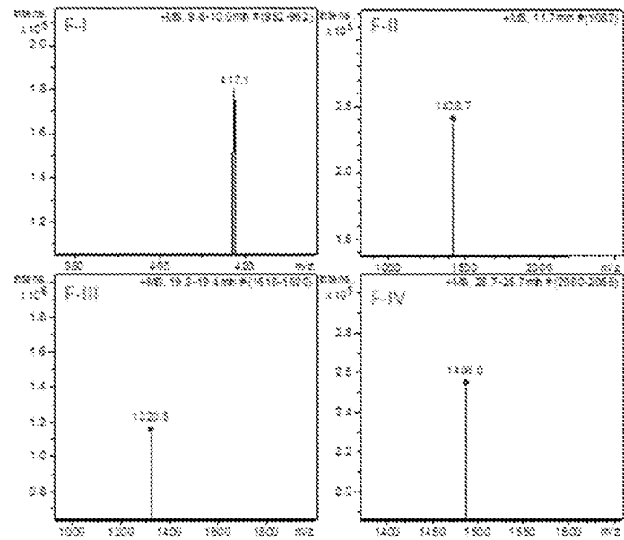
Figure 10: Four fragments of Insulin Glargine after digestion
