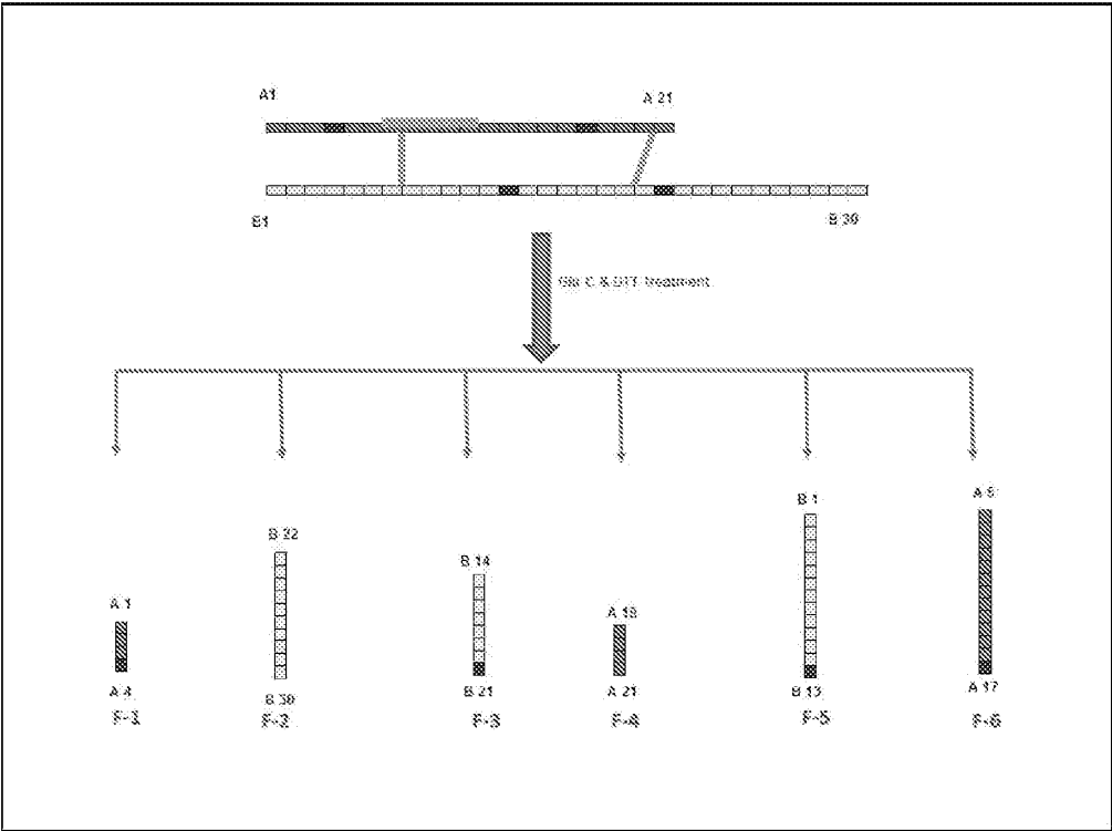
Figure 4: Insulin – Peptide fragments after Digestion and Reduction
