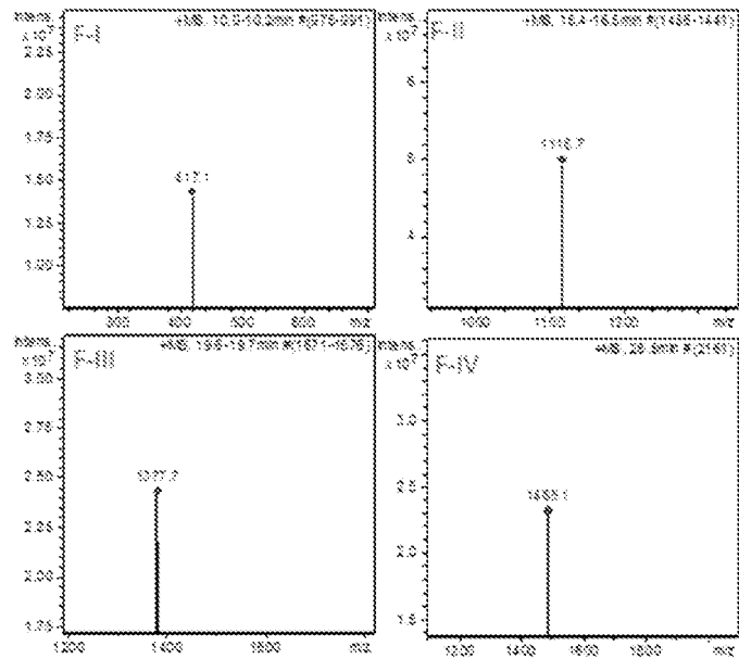
Figure 9: Four fragments of Human Insulin after digestion
