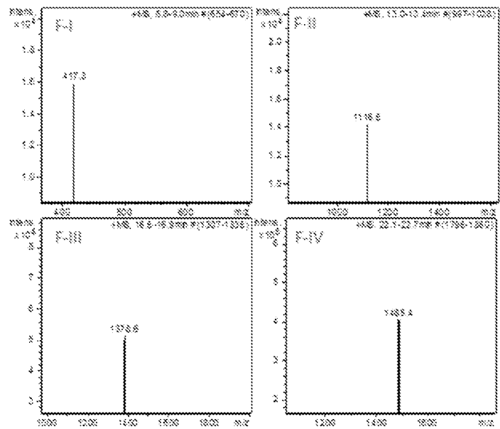
Figure 12: Four fragments of Insulin Lispro after digestion
