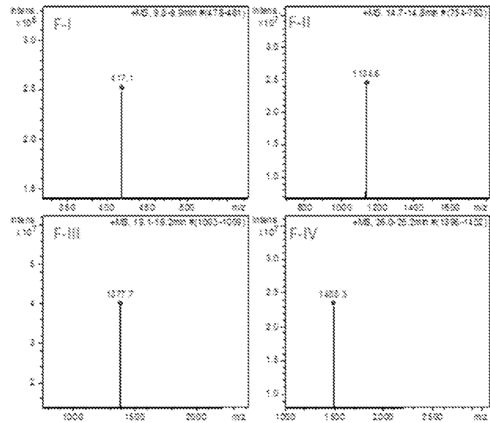
Figure 11: Four fragments of Insulin Aspart after digestion
