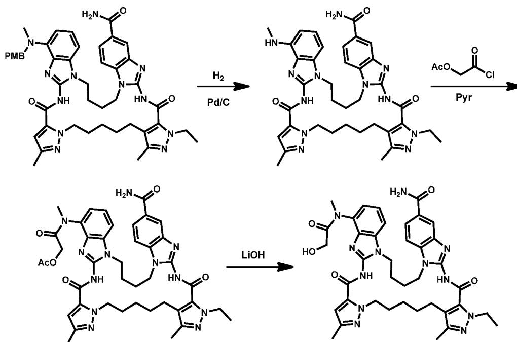
Example 48
