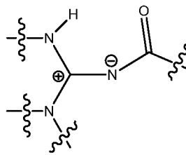
Formula (E)
