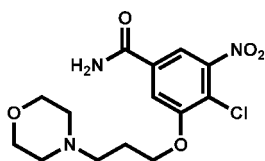
Step 1: 4-Chloro-3-(3-morpholinopropoxy)-5-nitrobenzamide
