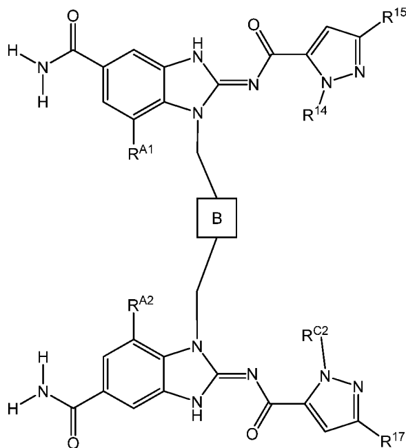
Formula (I-P-b')
