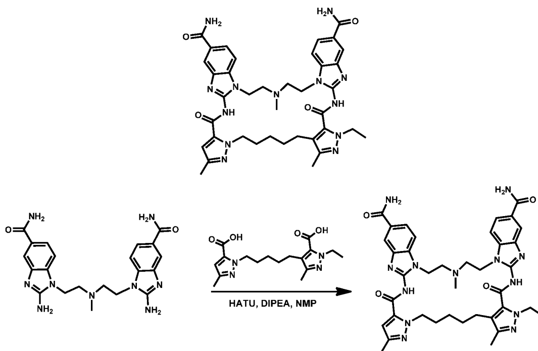
Example 8
