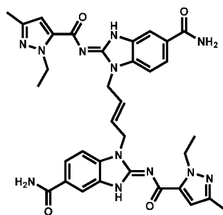
Example 3
