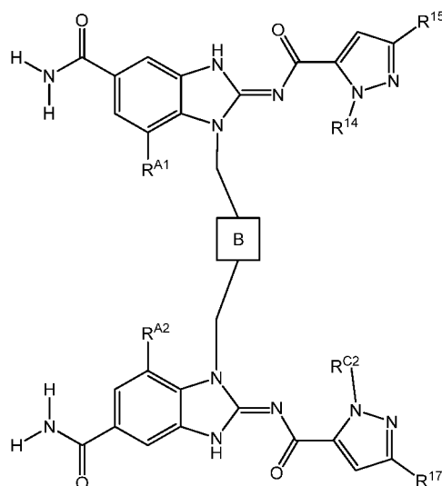
Formula (I-N-b')
