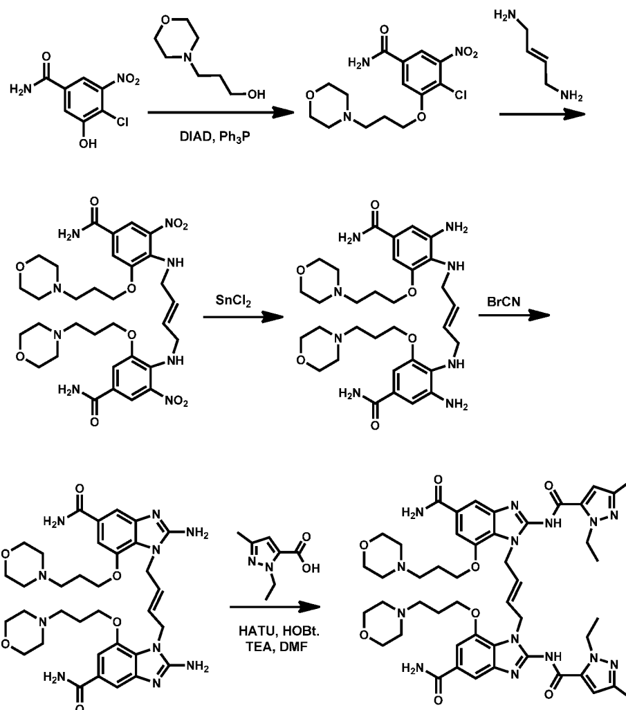
Step 1: 4-Chloro-3-(3-morpholinopropoxy)-5-nitrobenzamide
