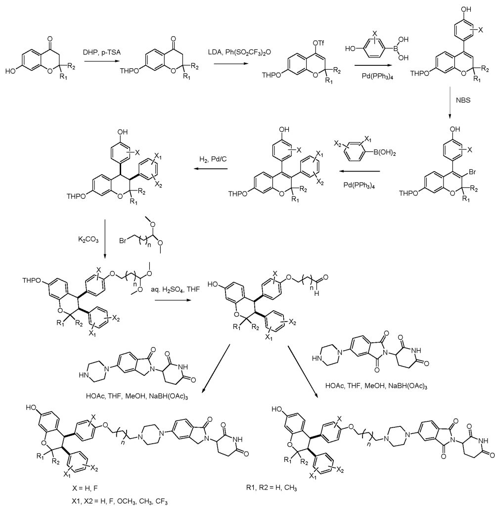
Scheme 8: Synthesis of Compounds 26, 28-31
