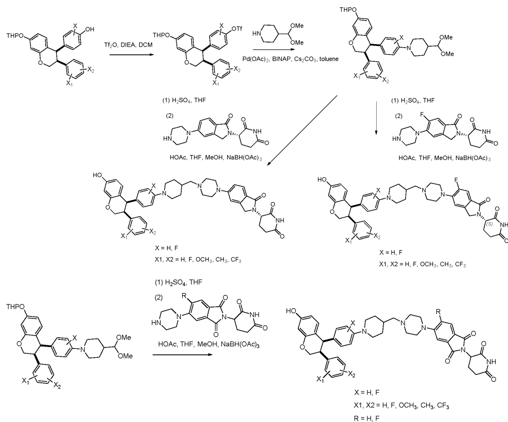
Scheme 12: Synthesis of Compounds 38-43, 45, 50-57, 60-65, 72-80, 84-87 and 89-90.
