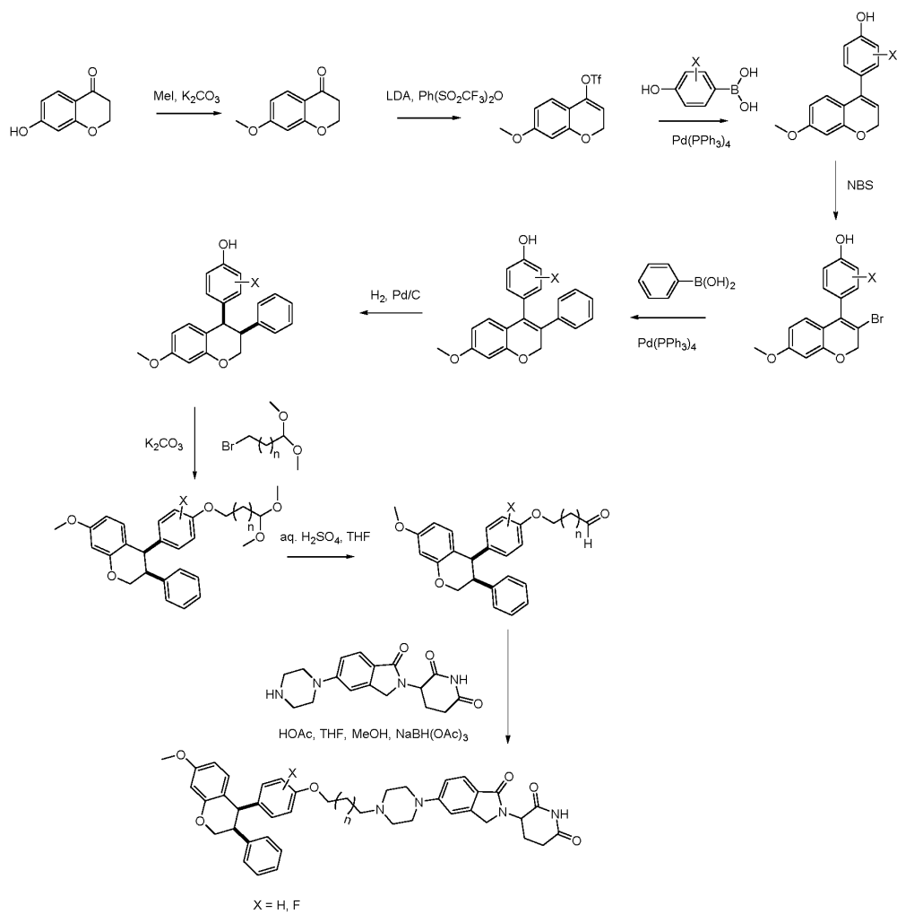
Scheme 9: Synthesis of Compound 27
