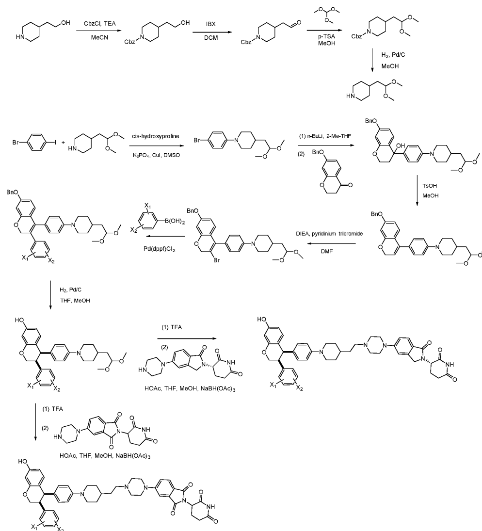
Scheme 11: Synthesis of Compounds 37 and 44.
