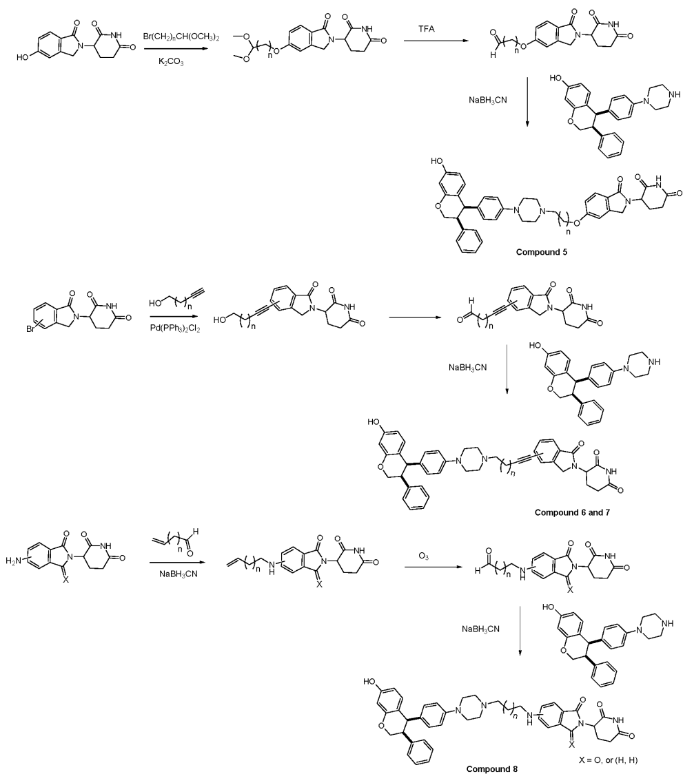
Scheme 5: Synthesis of Compounds 5-8
