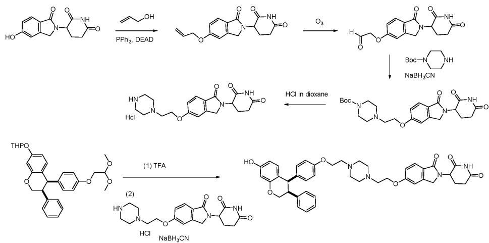
Scheme 3: Synthesis of Compound 3
