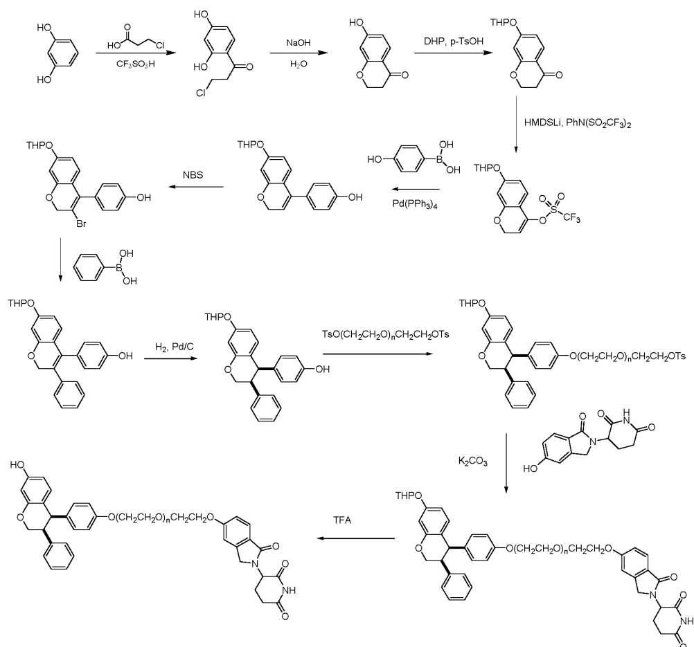
Scheme 1: Synthesis of Compound 1
