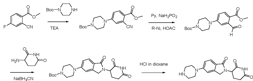
Scheme 7: Synthesis of Compounds 12-25
