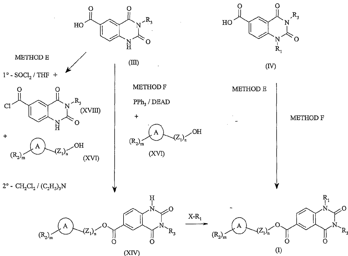
Scheme 8
