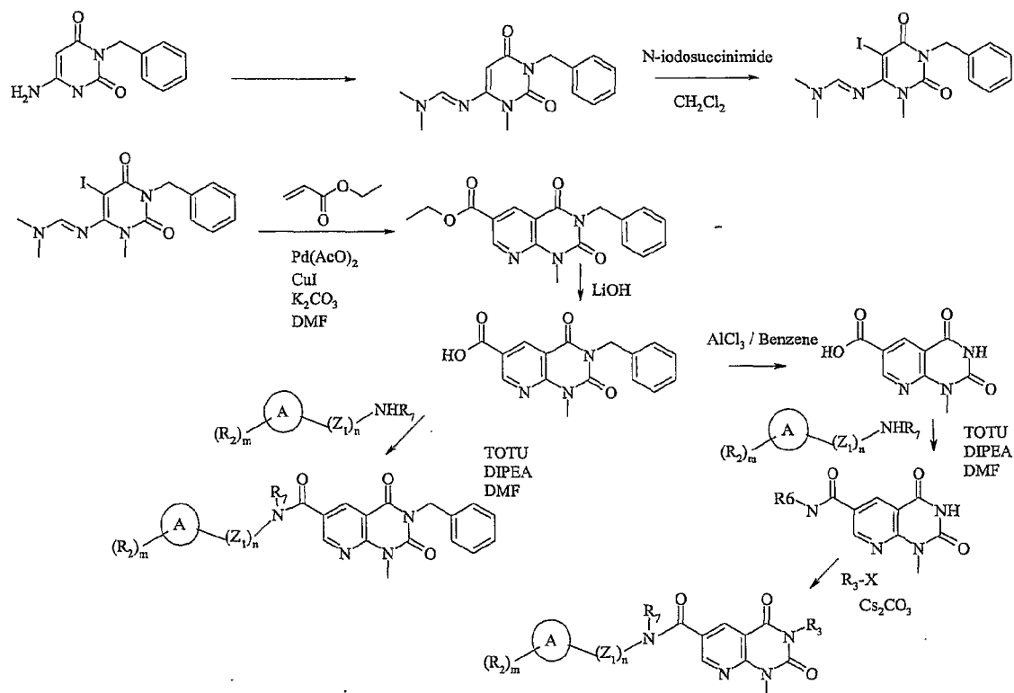
Scheme 10
