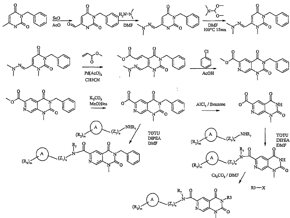
Scheme 11
