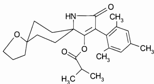
\beta isomer
