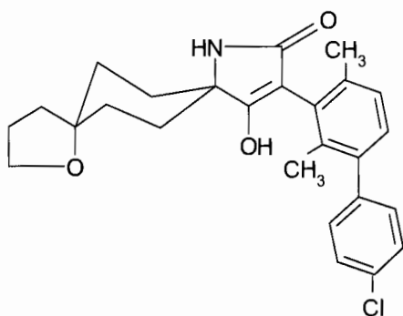
I-1-a-1
