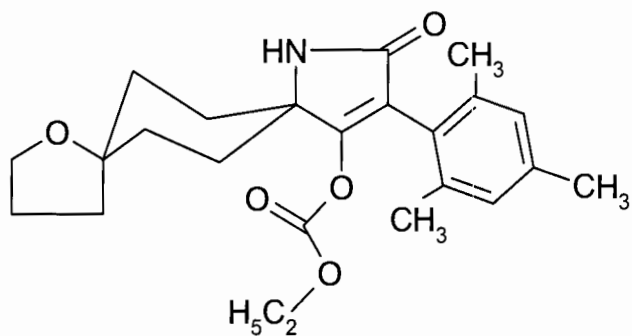
\beta isomer
