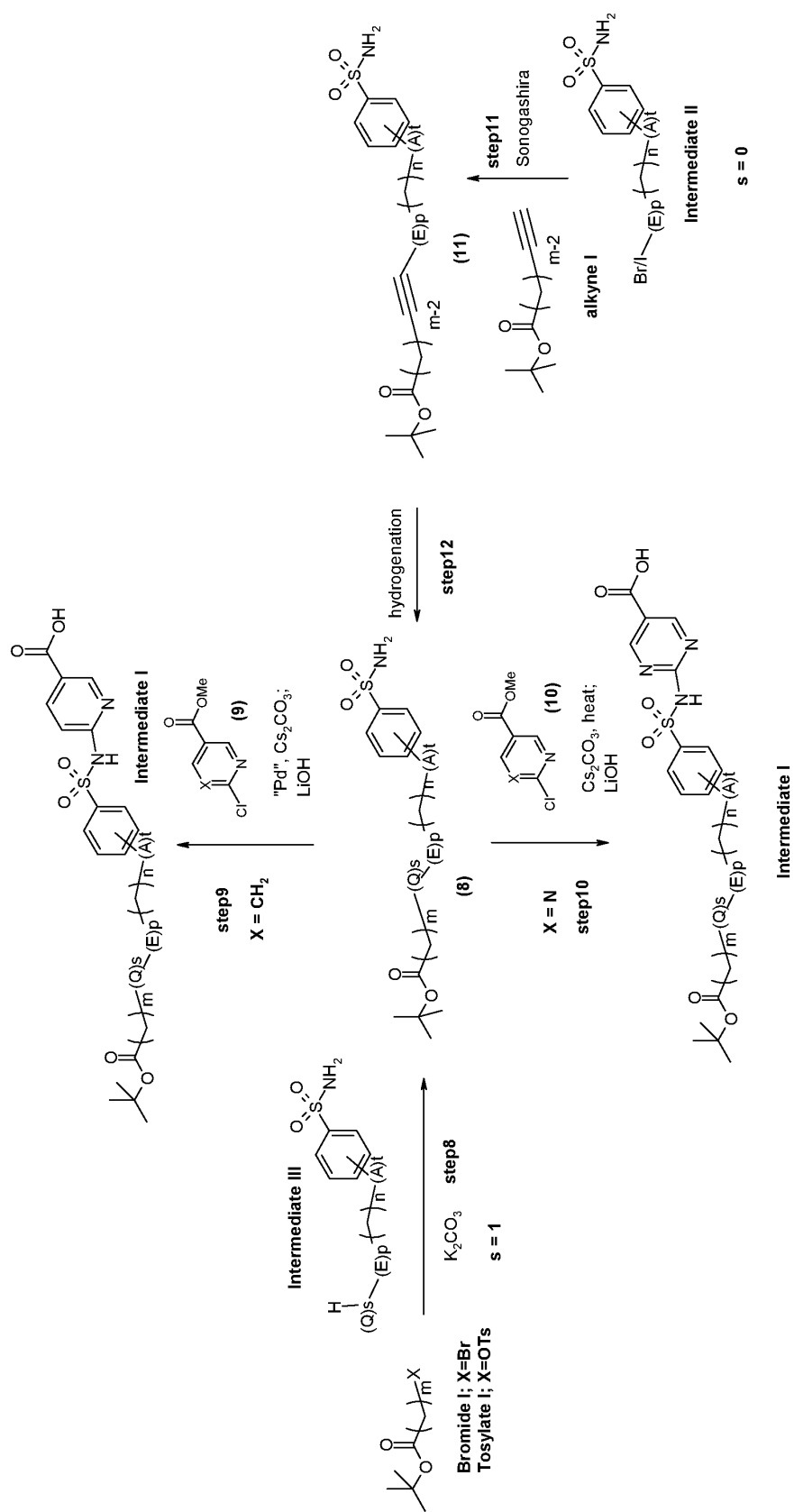
Scheme 2
