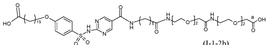
(I-1-2b)
