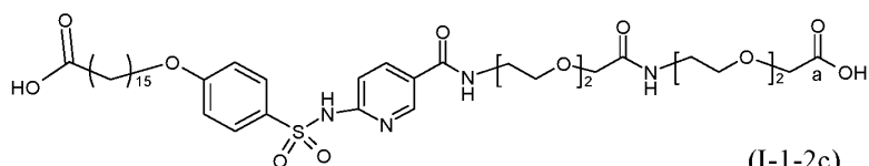
(I-1-2c)
