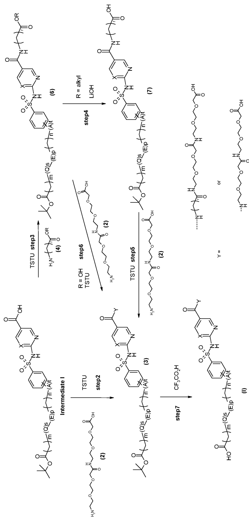
Scheme 1
