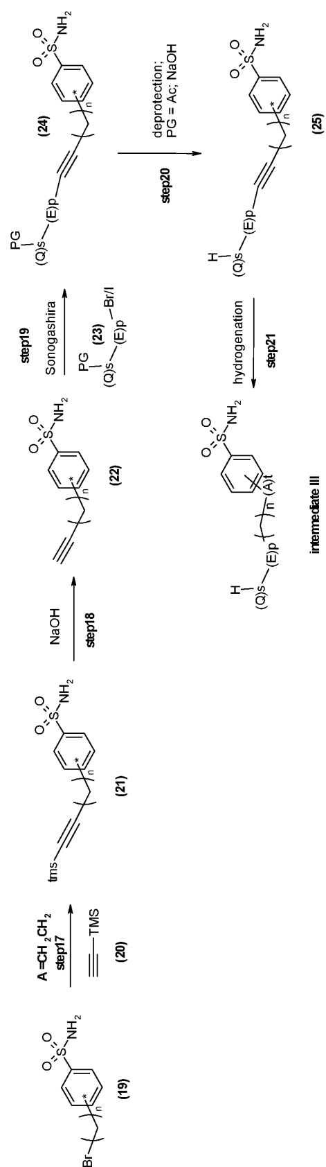
Scheme 4
