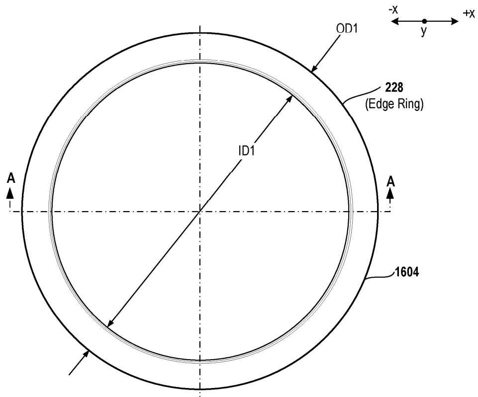
FIG. 8B (Top View)
