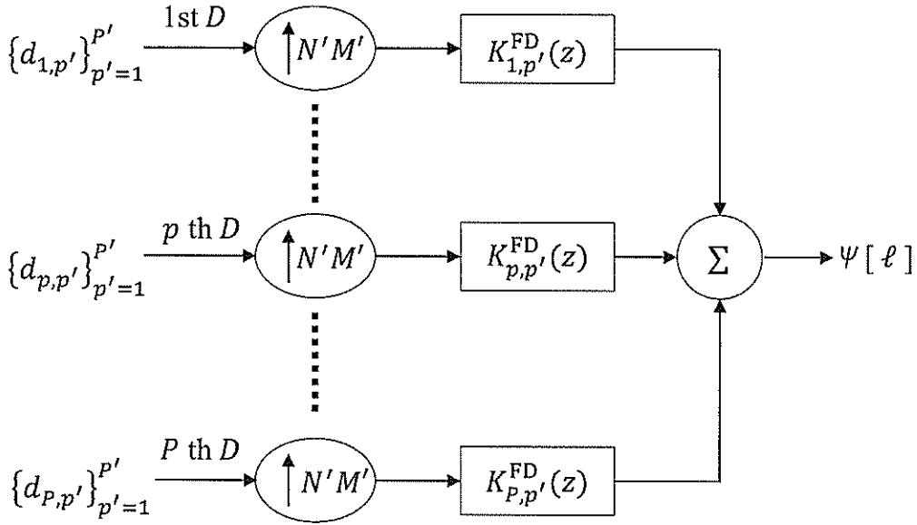
SFB for data embedded transmit FD signal
