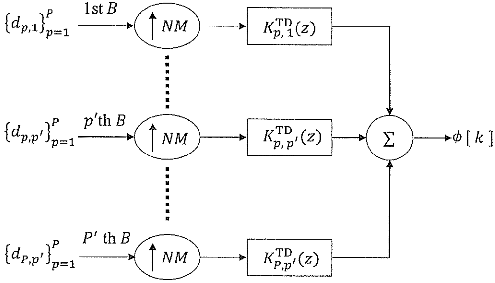
SFB for data embedded transmit TD signal
