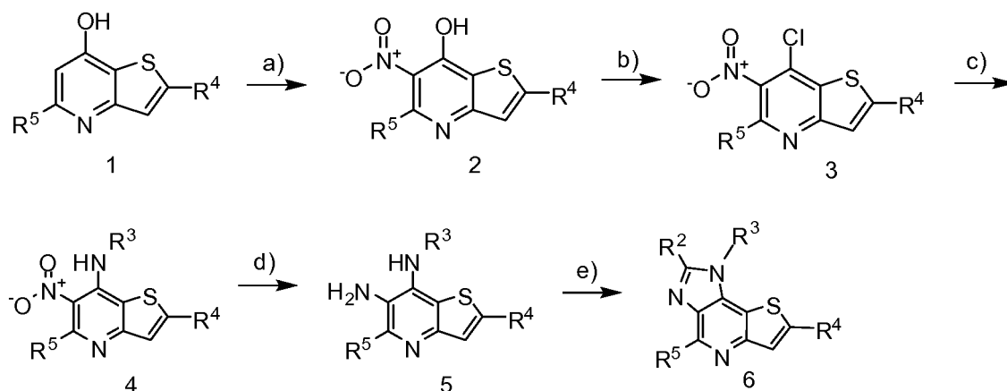
Scheme 1
