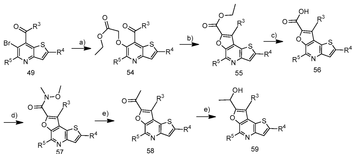
Scheme 11
