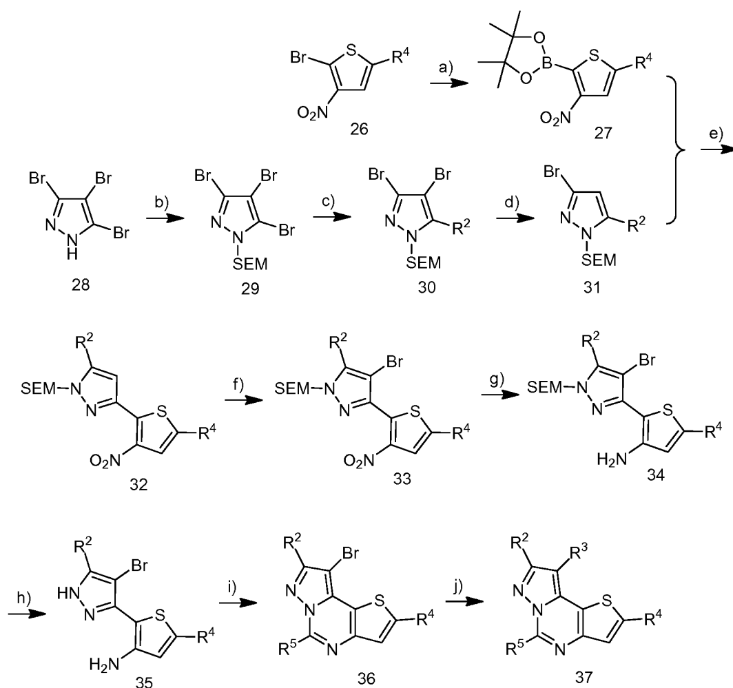
Scheme 7
