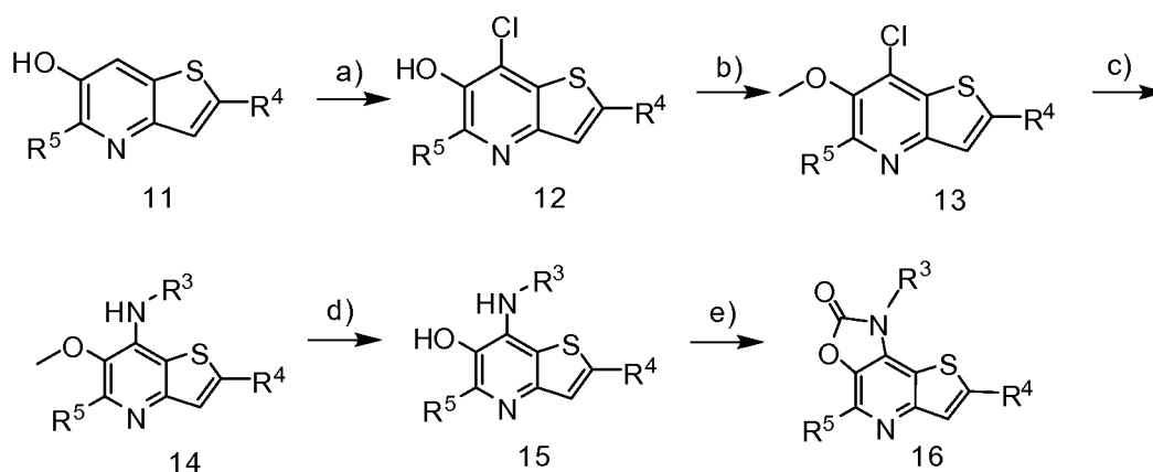
Scheme 3
