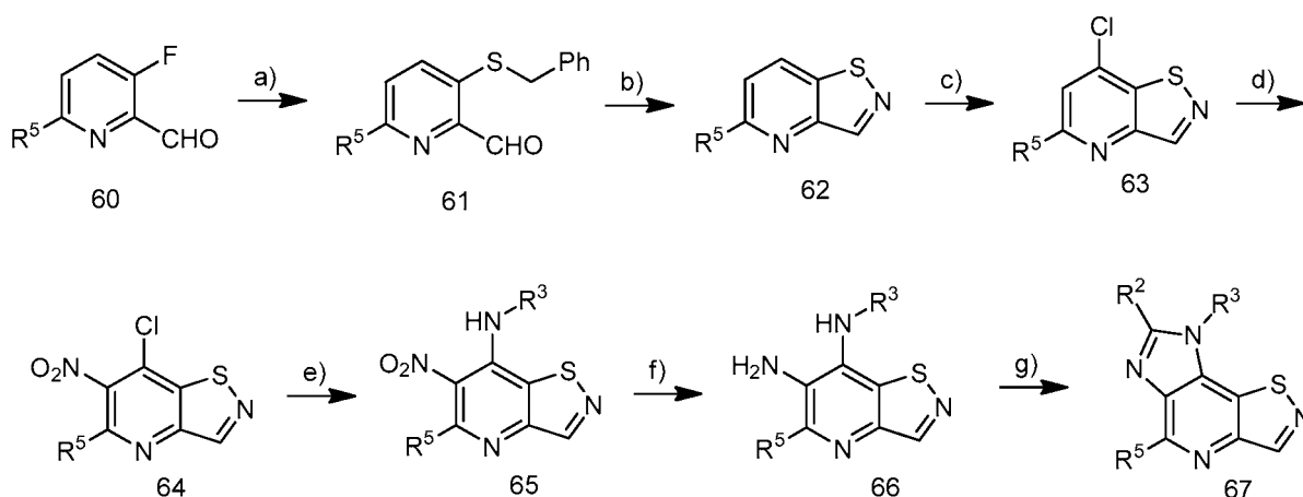
Scheme 12
