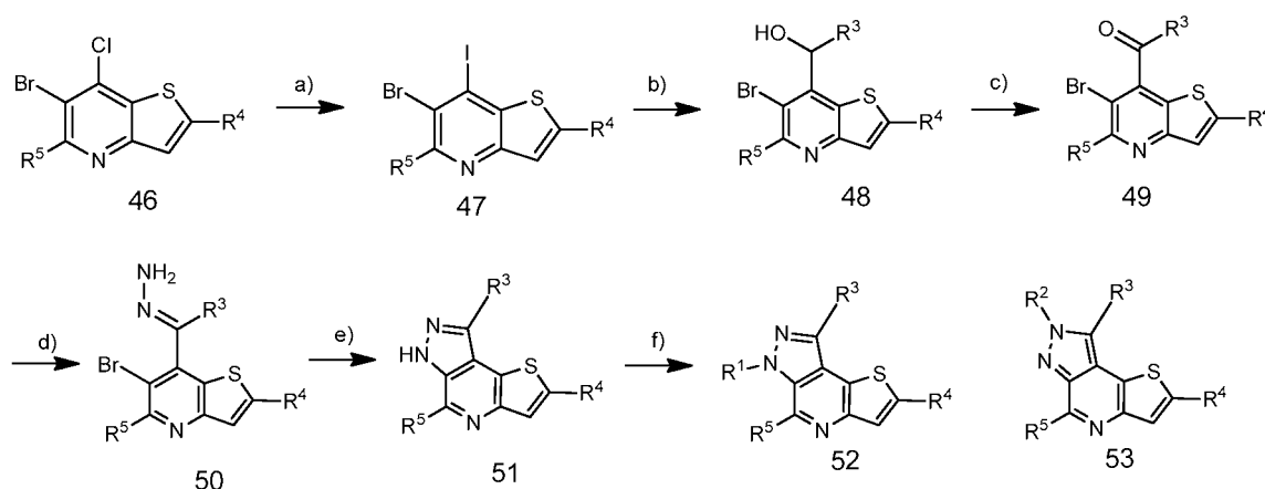
Scheme 10
