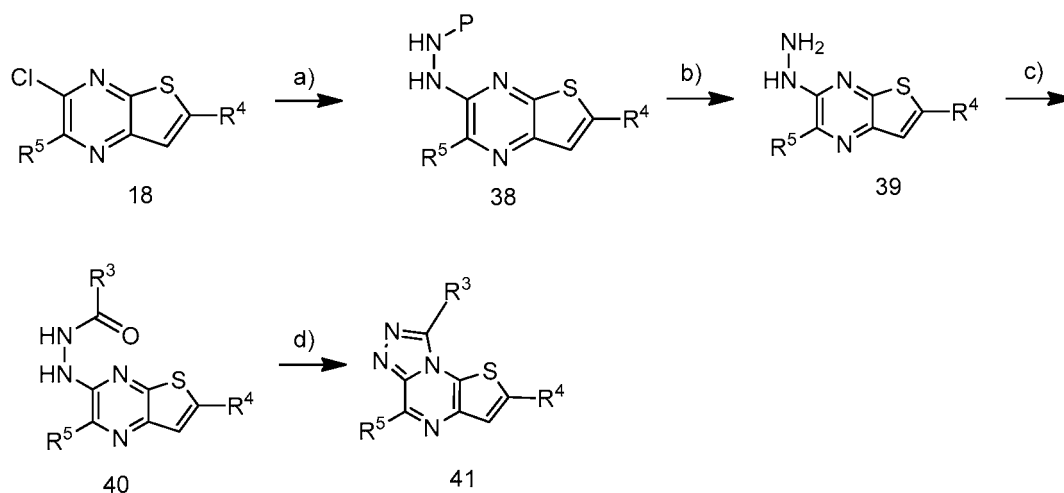
Scheme 8
