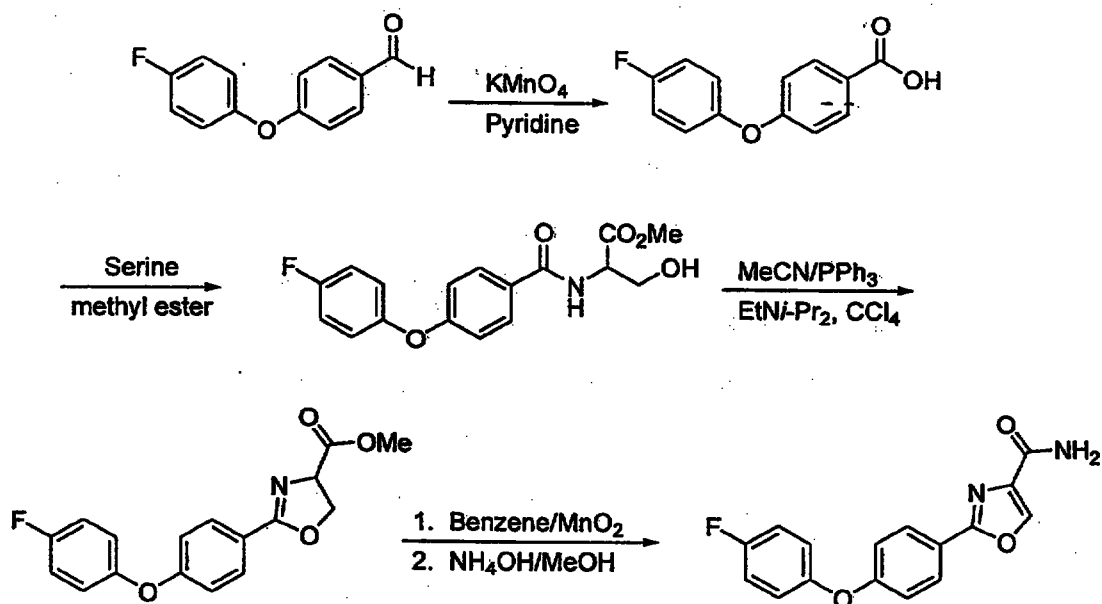
Scheme 7
