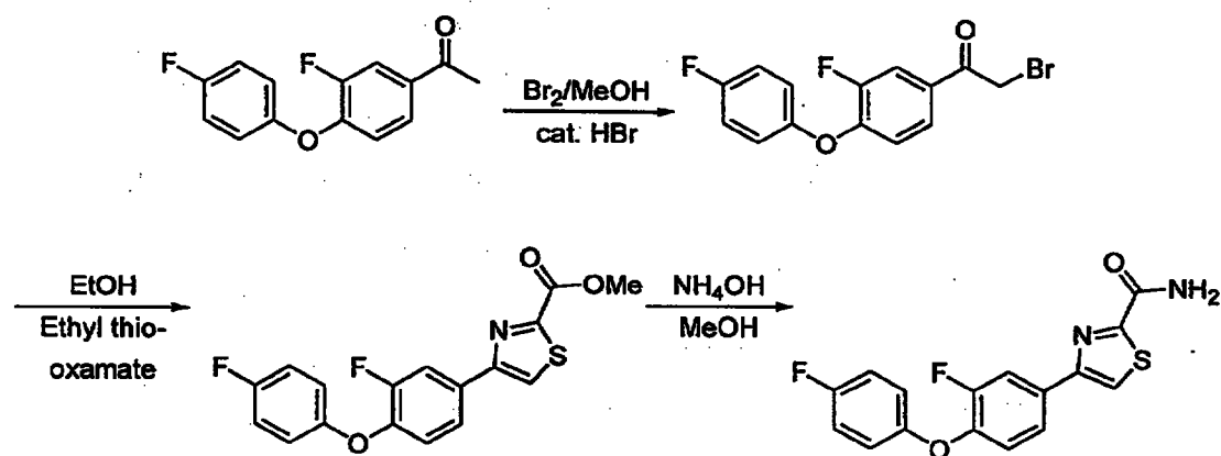
Scheme 8
