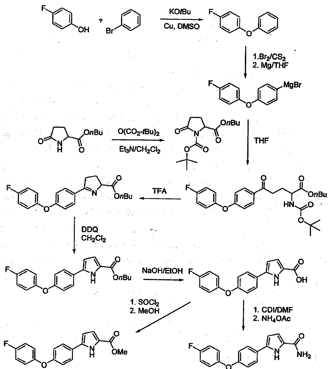
Scheme 6
