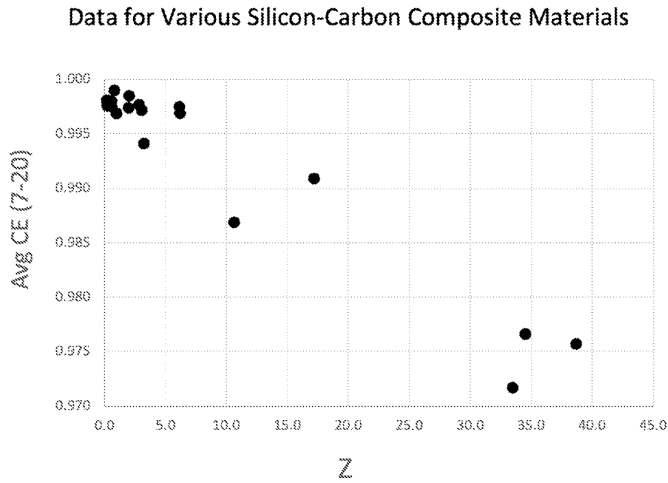
Relationship between Z and average Coulombic efficiency for various silicon-carbon composite materials.
