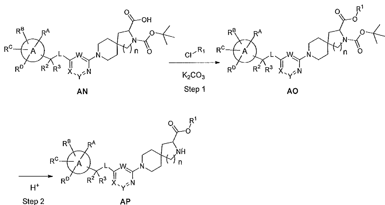
Scheme 9
