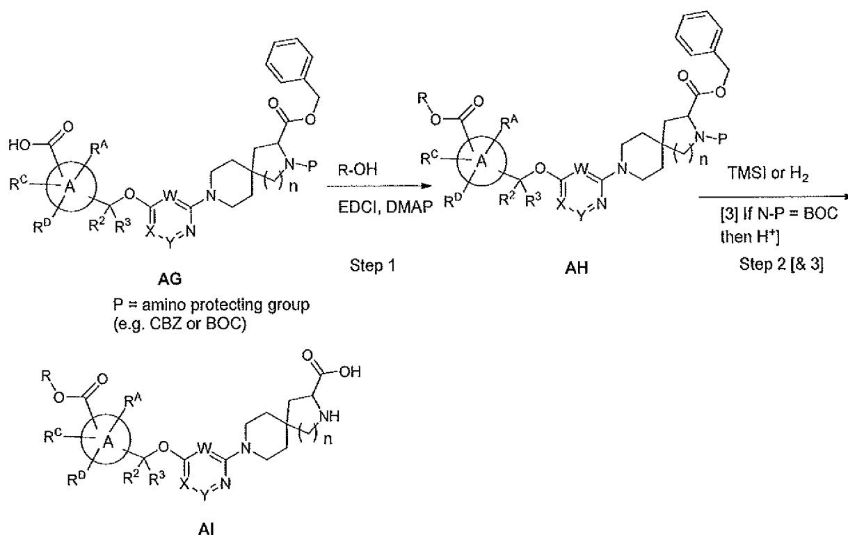
Scheme 6
