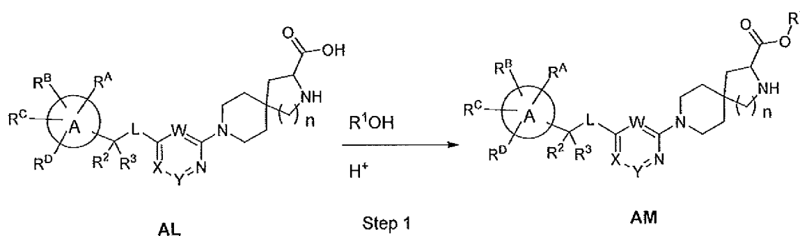
Scheme 8
