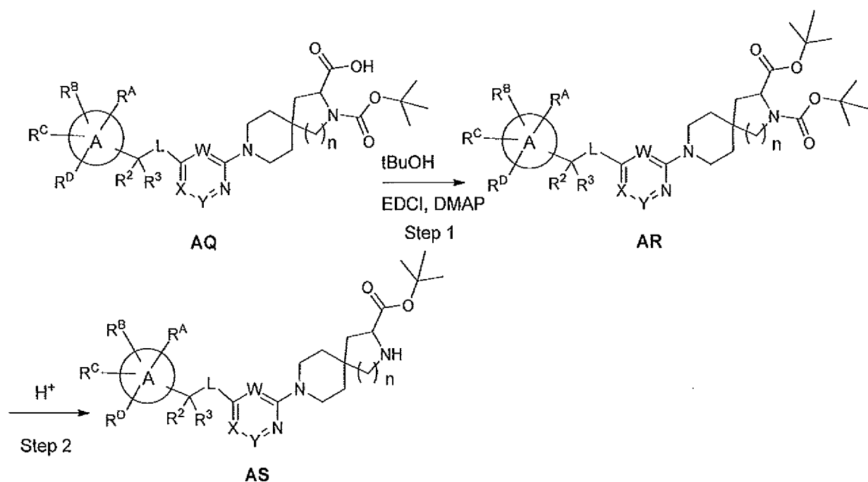
Scheme 10
