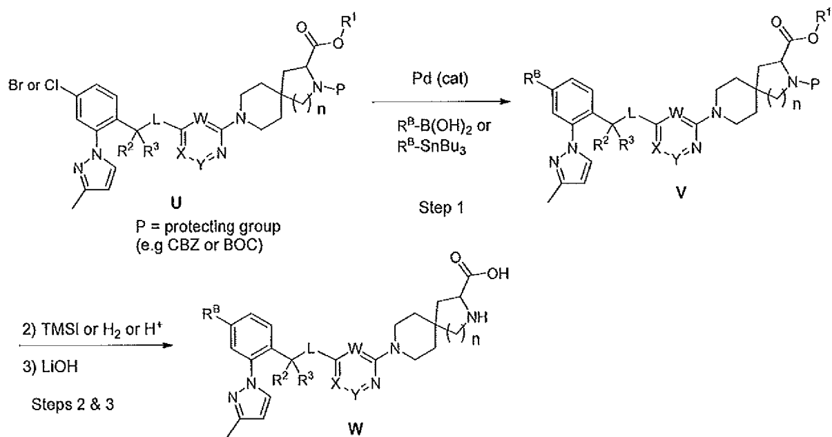
Scheme 4b
