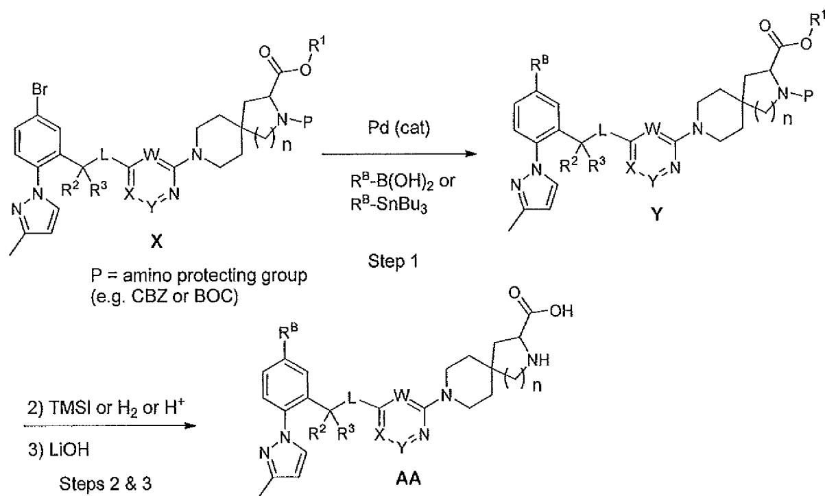
Scheme 4c
