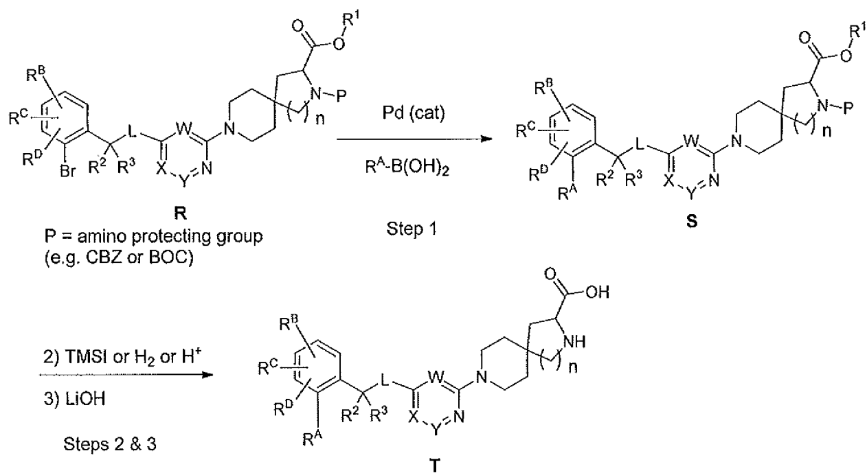
Scheme 4a
